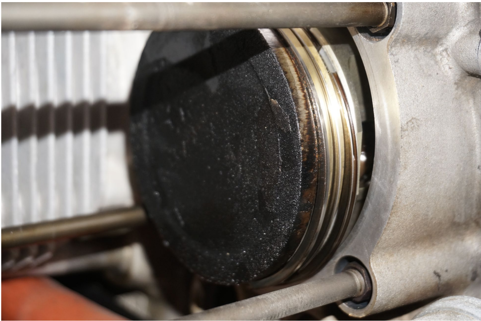
Photograph 9 - Side View of Piston
