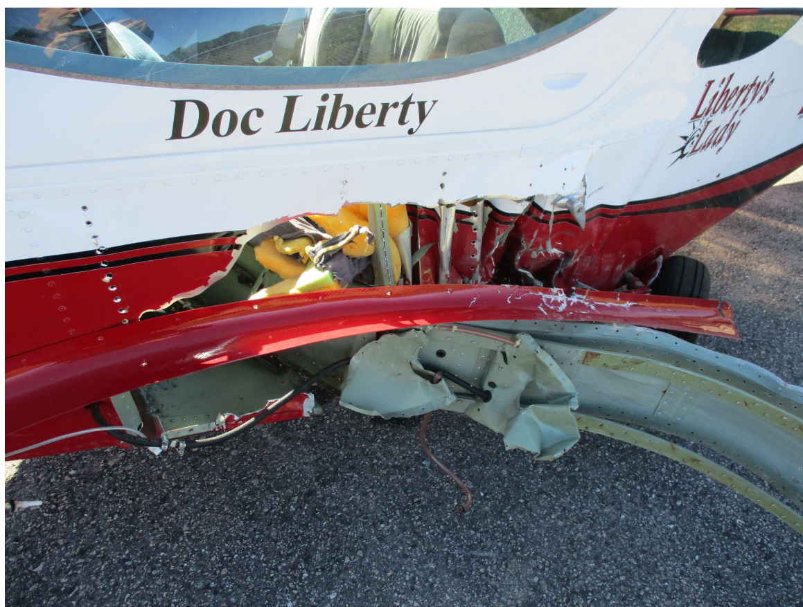
Photograph 3 - Close Up of Left Wing Root (Courtesy of FAA)
