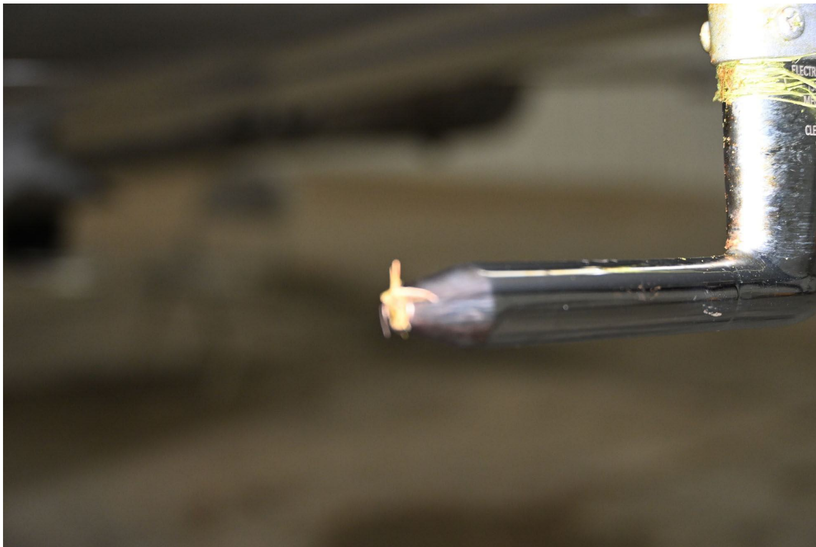
Photograph 6 - Pitot tube with tree material plugging the pitot hole (Courtesy of Cirrus)
