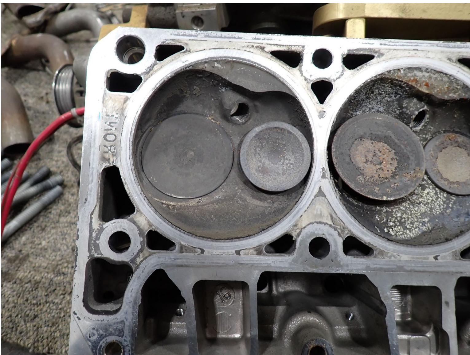
Photograph 11 - No. 1 cylinder head with valves
