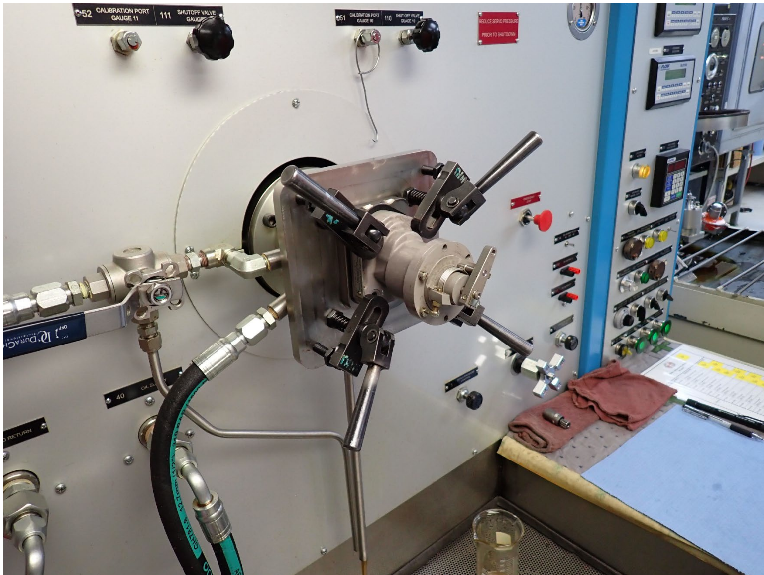
Photograph 4 - Propeller governor on test bench (Courtesy of Hartzell)
