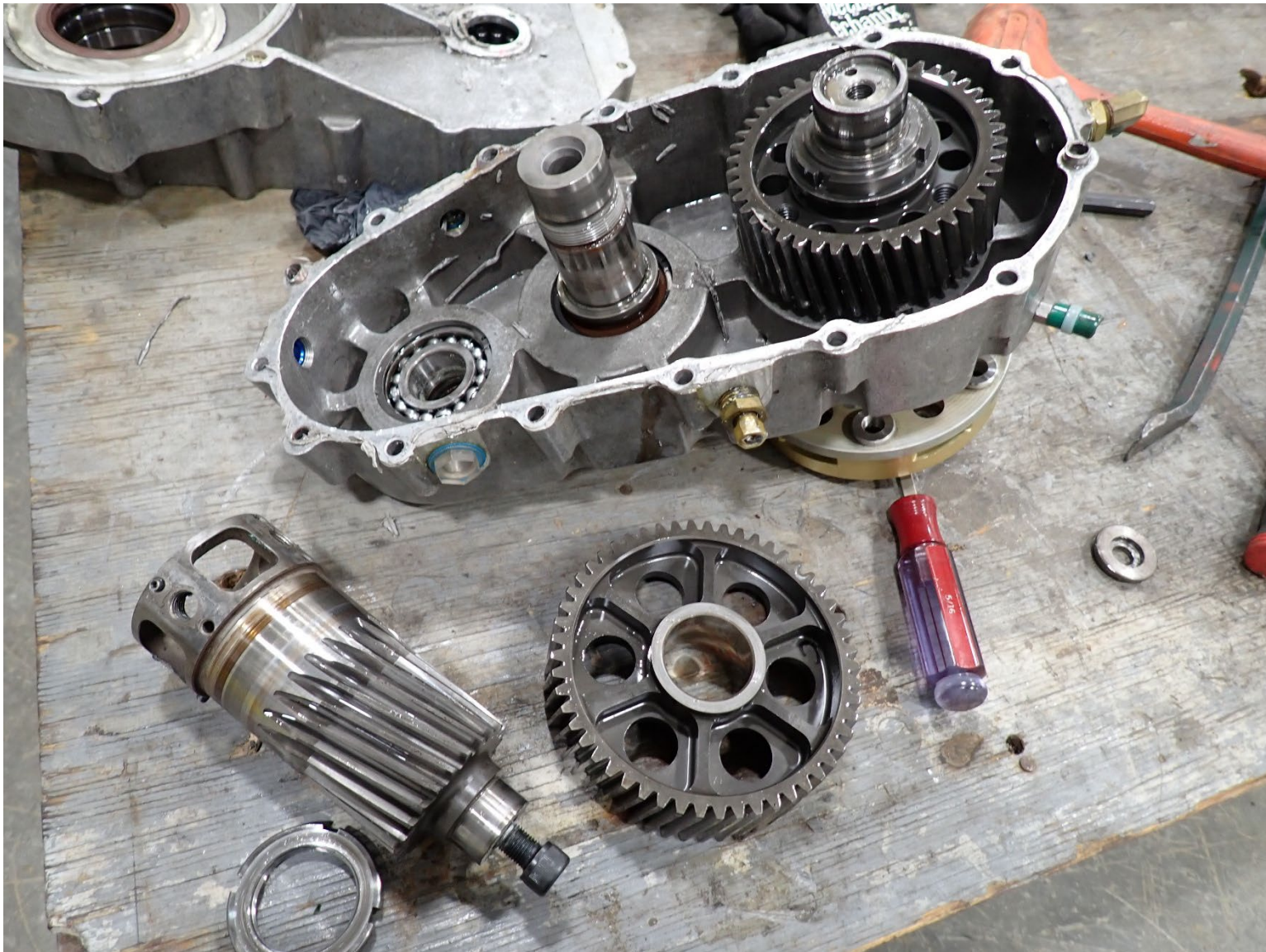
Photograph 12 - Propeller gearbox after disassembly
