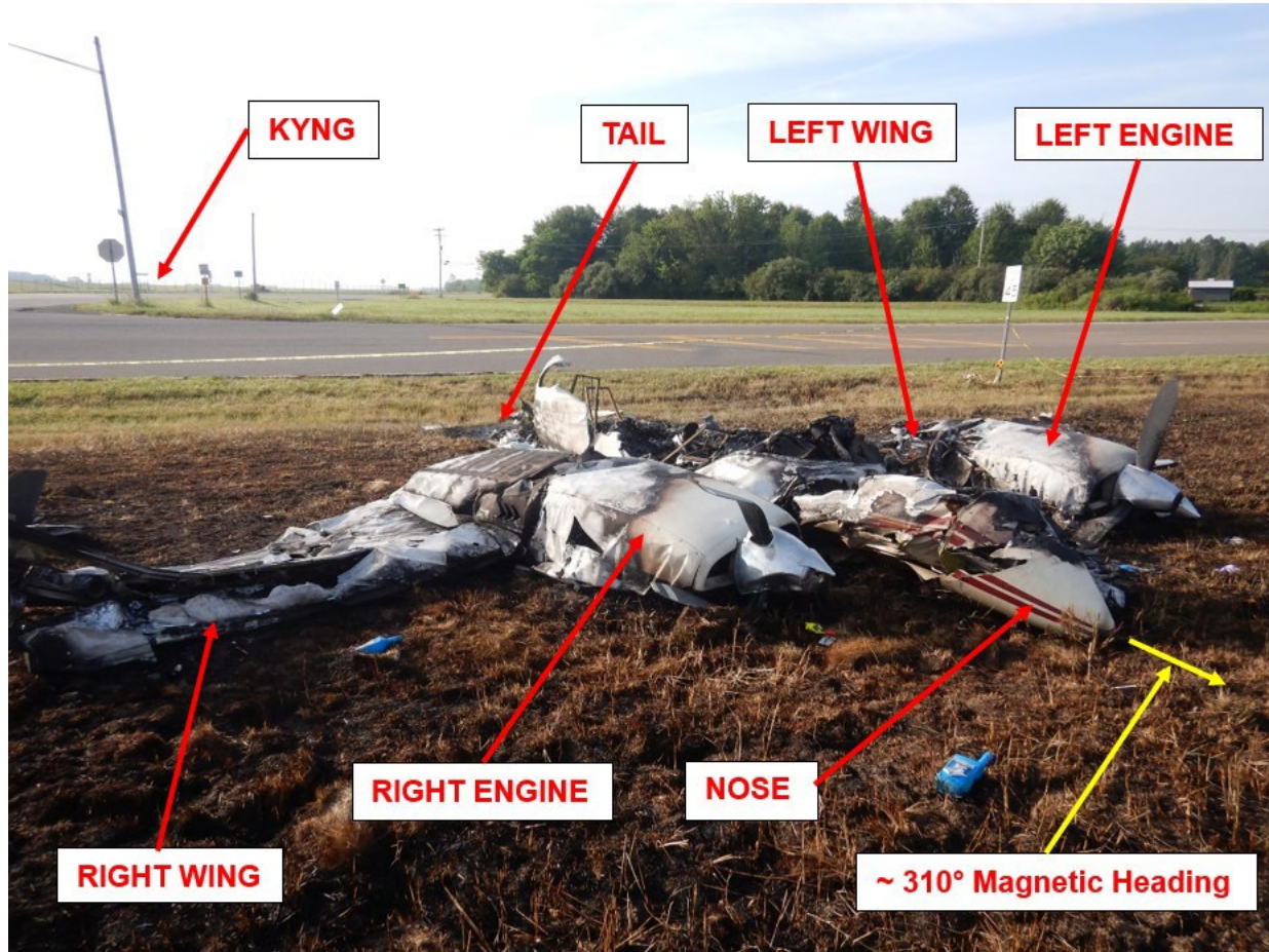
Wreckage Diagram (Courtesy of Textron Aviation)
