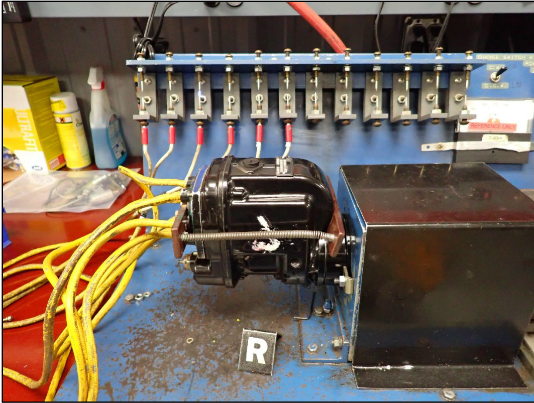
Figure 2: View of right magneto on test stand.
