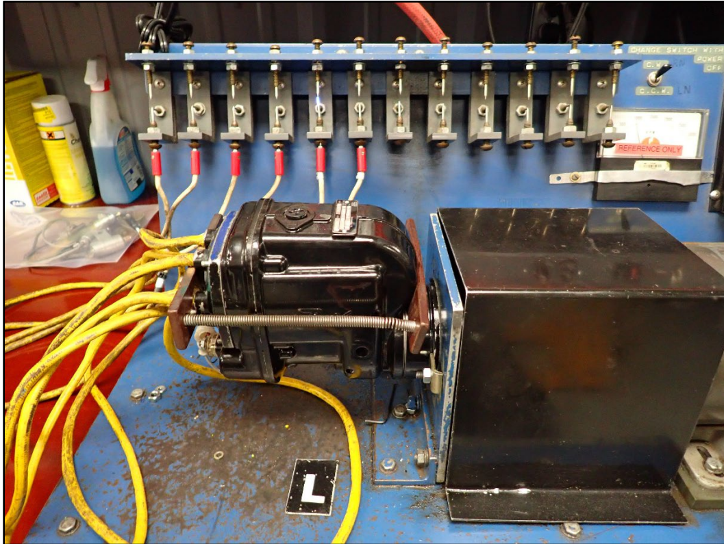
Figure 1: View of left magneto on test stand.
