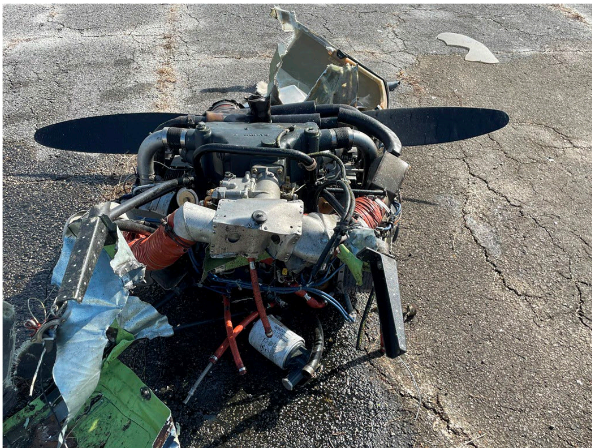
Photograph 4 - Right Engine at Accident Site
