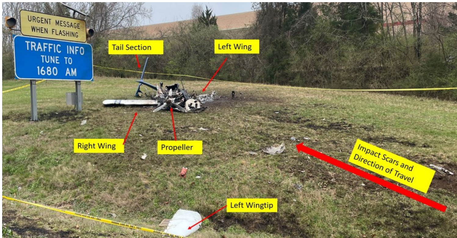
Photograph 5 - Wreckage site diagram. (NTSB)
