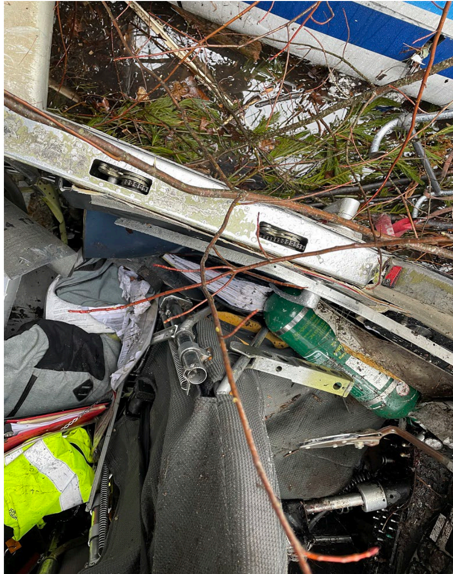
Photograph 3 - Cockpit Door/Hatch Handles And Latches as Found (Courtesy of FAA)
