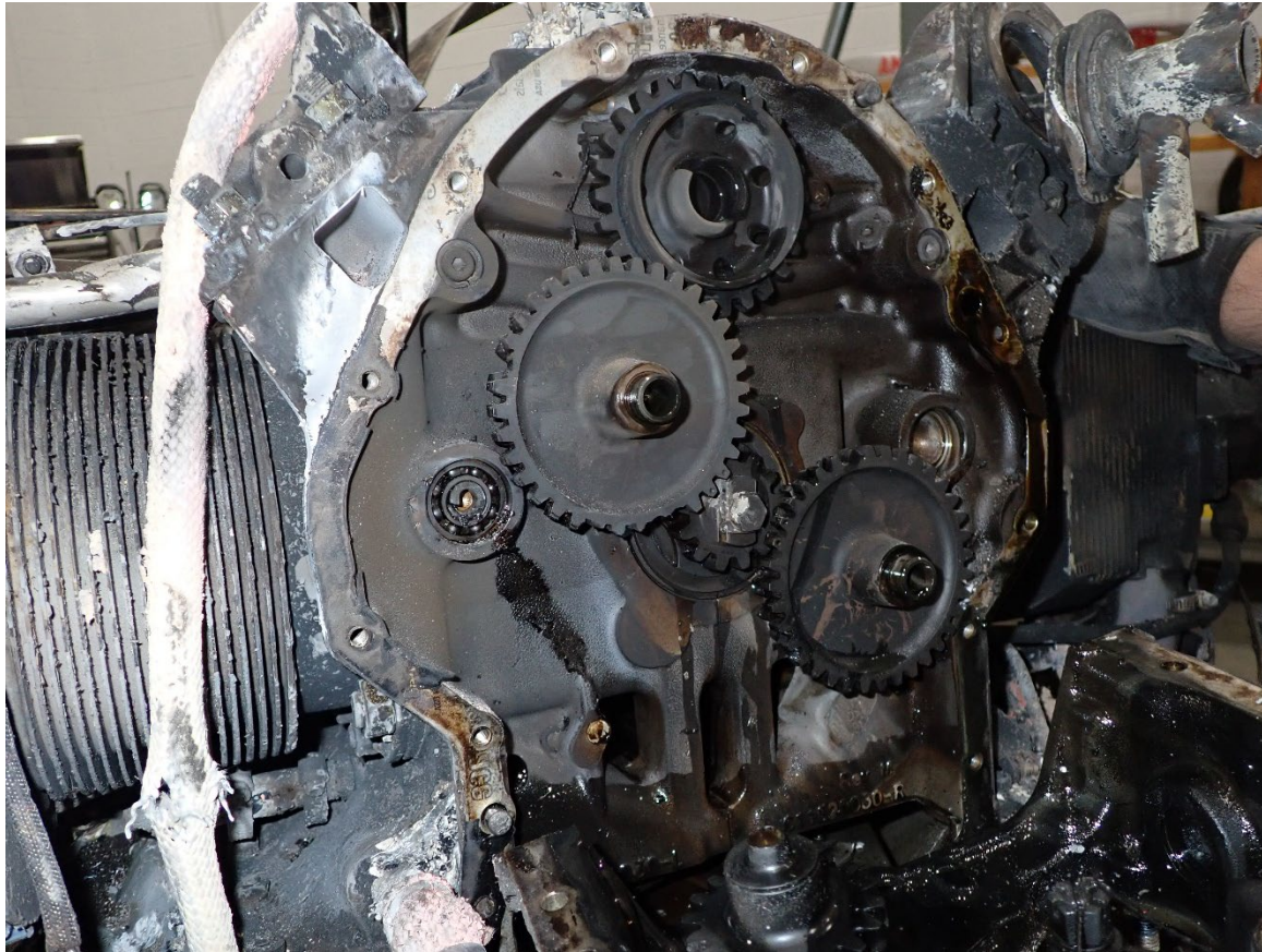
Photograph 15 - NTSB Digital Photograph. View of the Accessory Section of the Engine Following Removal of the Accessory Case
