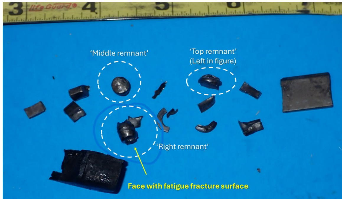
Photograph 21 - NTSB Digital Photograph. Annotated photograph depicting pieces of Impulse Coupling Rivet Found in Oil Sump
