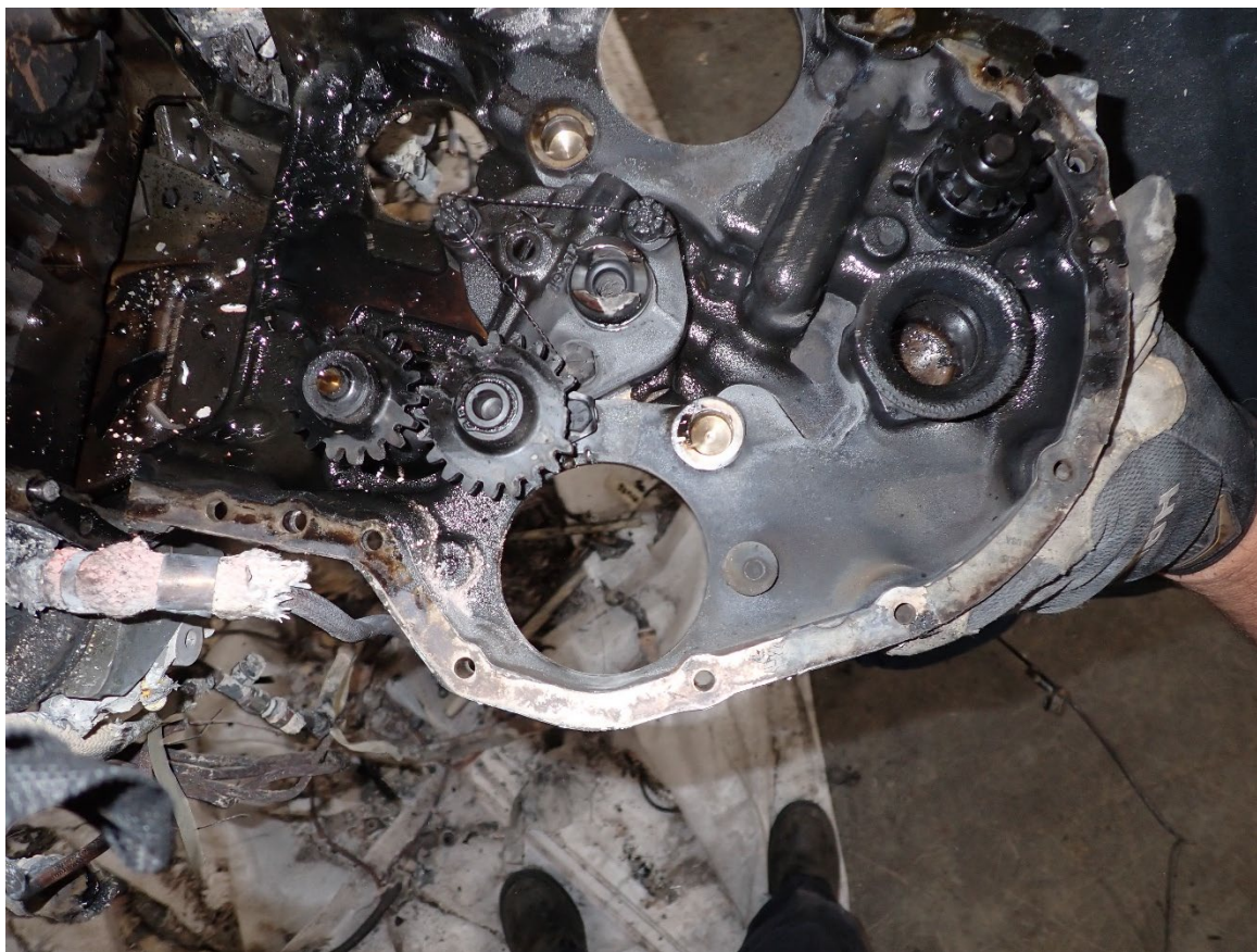
Photograph 16 - NTSB Digital Photograph. View of the Accessory Case Following Removal From the Engine
