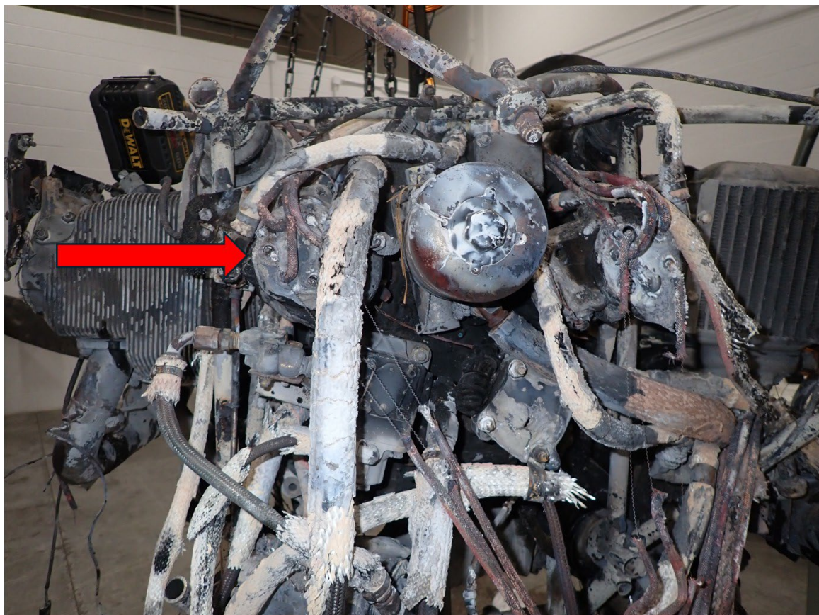
Photograph 12 - NTSB Digital Photograph. Arrow Points to Heat Damaged Left Magneto
