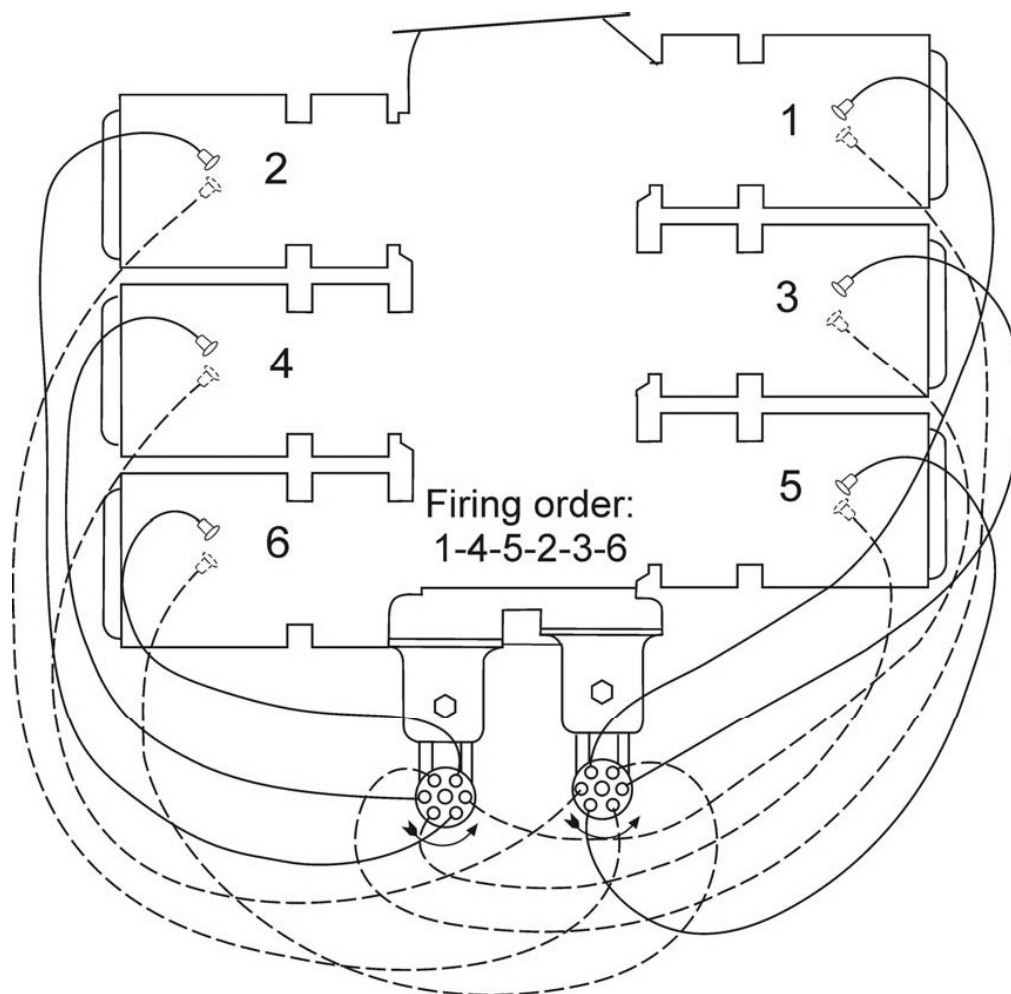
Figure 5-1. Ignition Wiring Diagram
