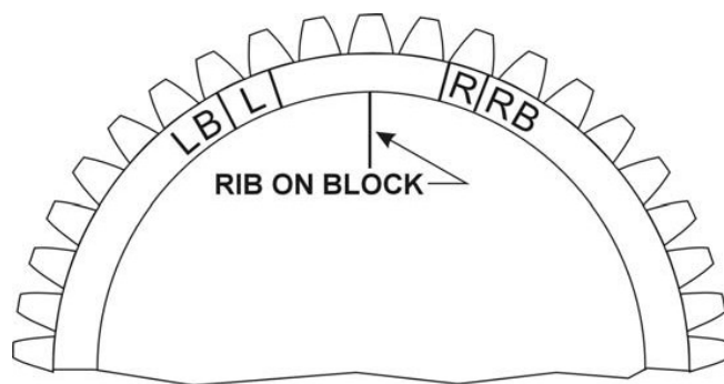
Figure 5-2. Timing Marks – 6 Cyl. –1200 Series
