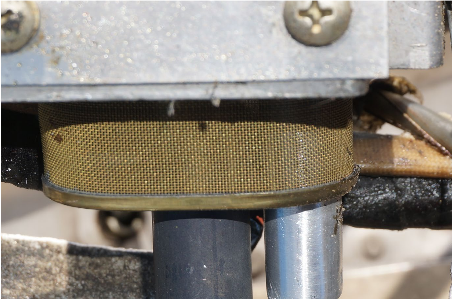
Photograph 35 - Fuel Strainer
