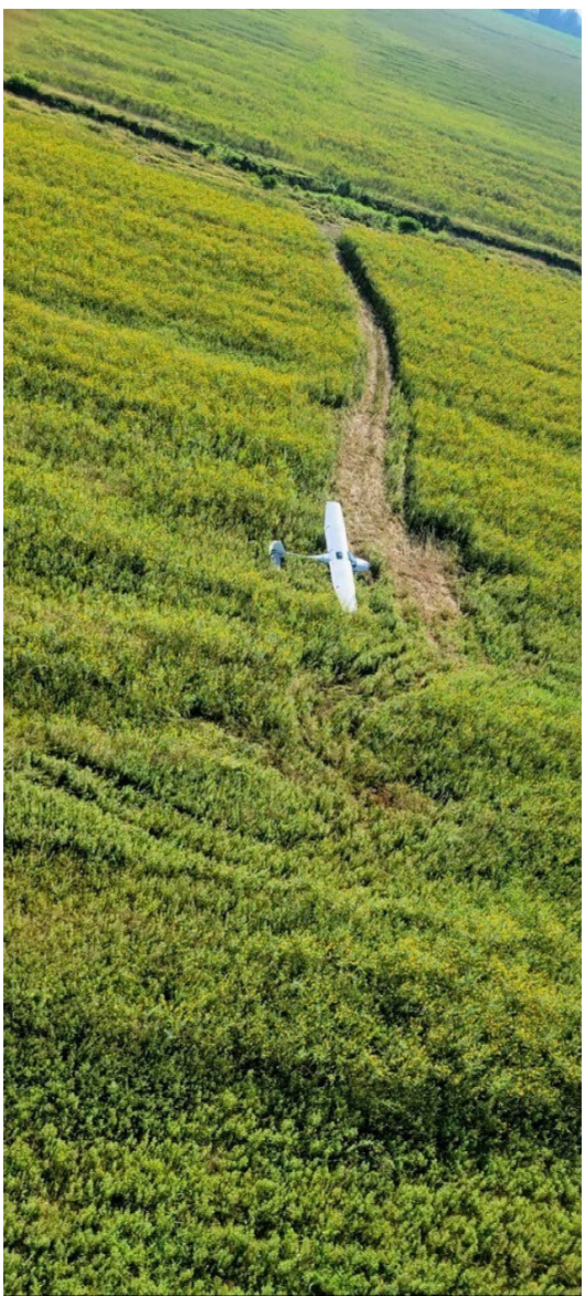
Photograph 2 - Aerial View of Main Wreckage (Courtesy of Florida Air Recovery)
