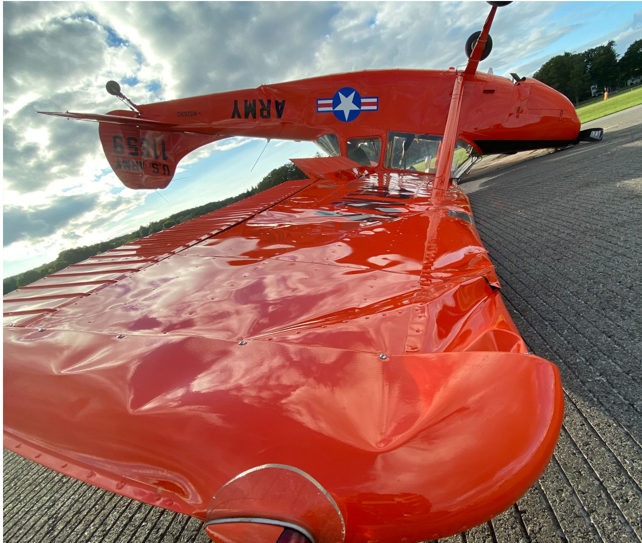
Photograph 3 - Closeup view of left wing damage (Courtesy of FAA)
