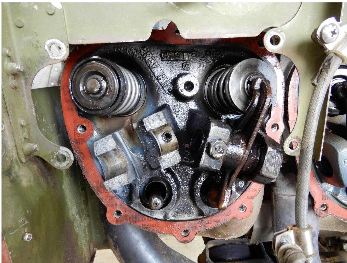
Photograph 7 - No. 6 Cylinder (NTSB Photo)
