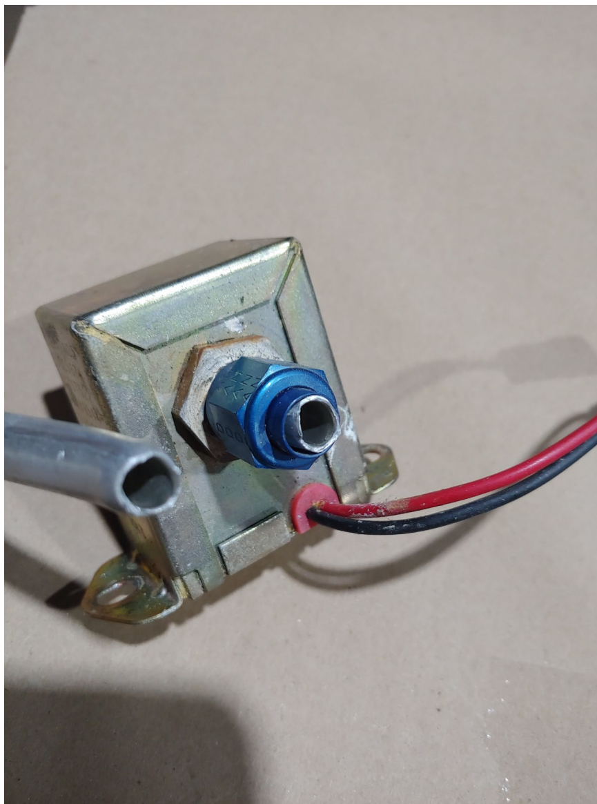
Photograph 8 - View of boost pump and fractured fuel line. (Courtesy of FAA)
