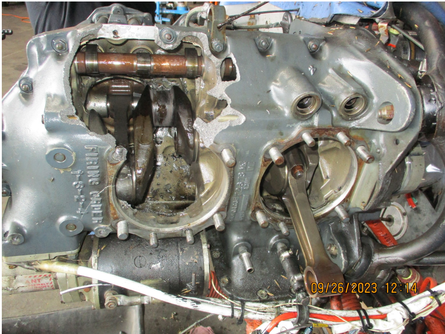
Photograph 3 - No. 2-4 cylinders removed.
