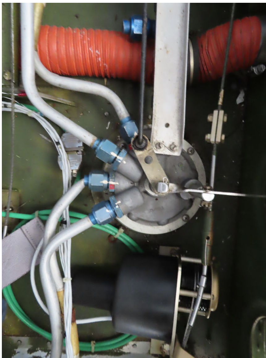
Photograph 4 - Fuel selector valve (Courtesy of Piper)
