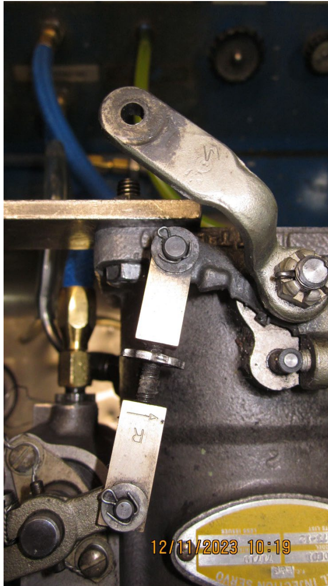
Photograph 3 - Mixture control linkage (Courtesy of FAA)
