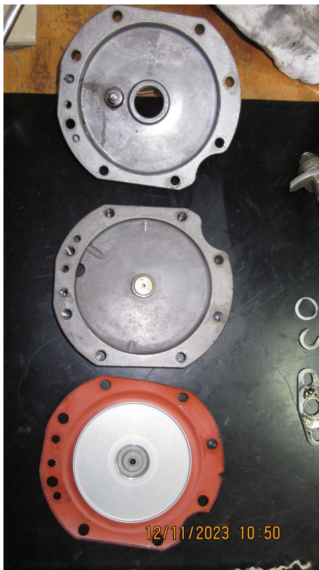
Photograph 5 - Fuel servo diaphragm and plates (Courtesy of FAA)
