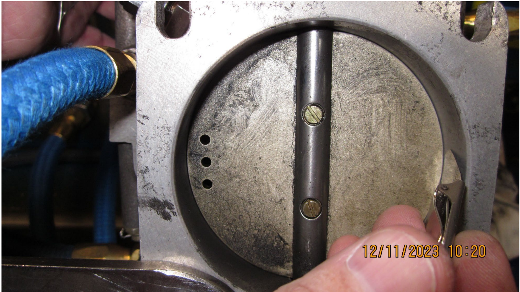
Photograph 4 - Throttle valve (Courtesy of FAA)
