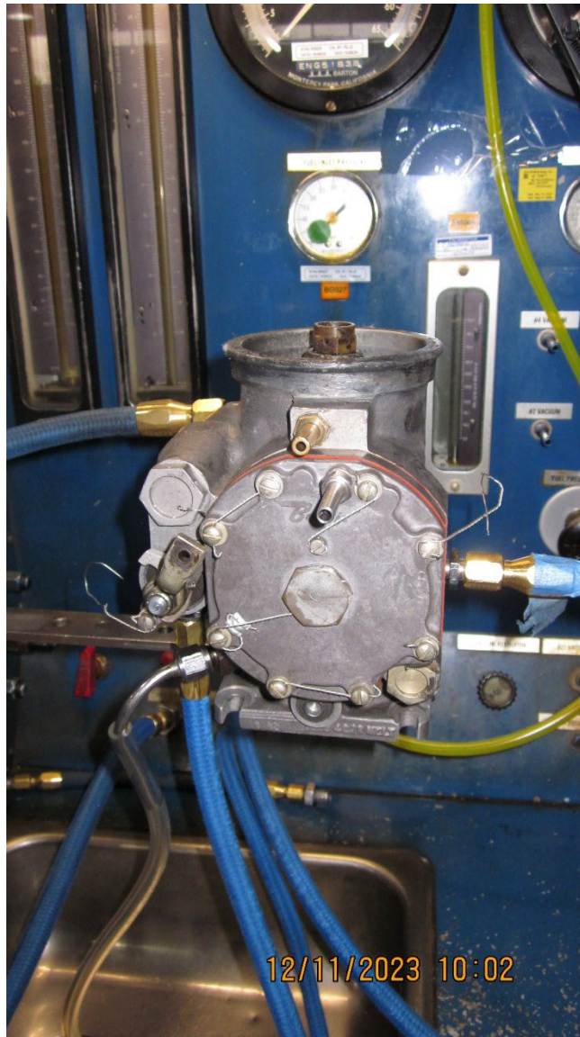
Photograph 1 - Fuel servo on test bench (Courtesy of FAA)
