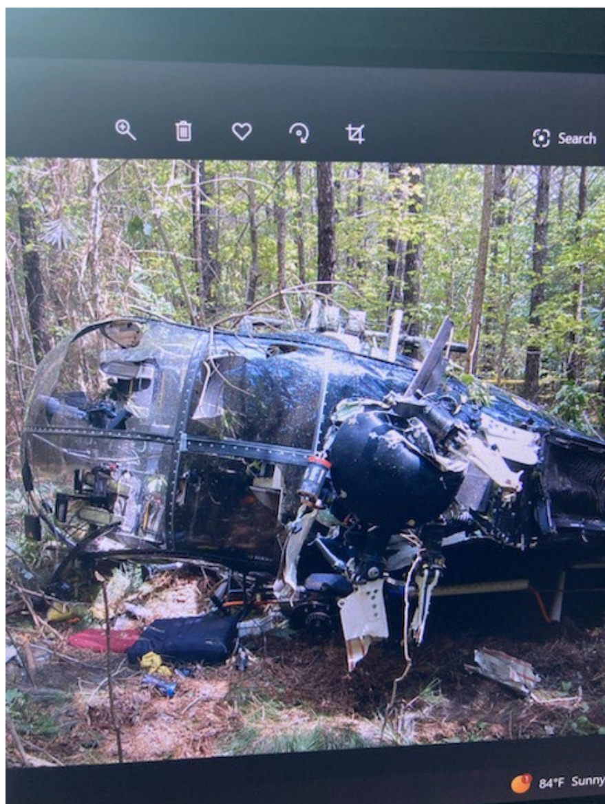
Photograph 2 - Main Wreckage (Courtesy of FAA)
