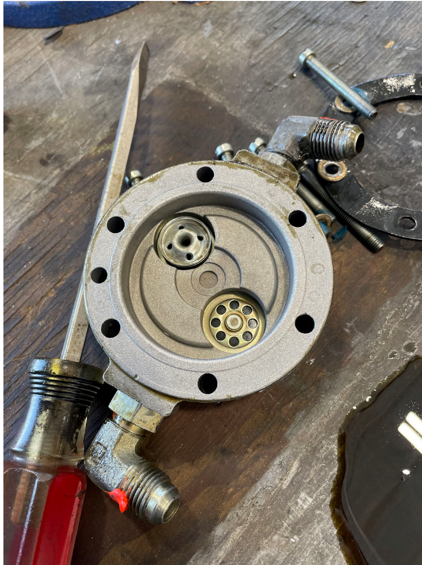
Photograph 6 - Engine-driven Fuel Pump (NTSB Photo)
