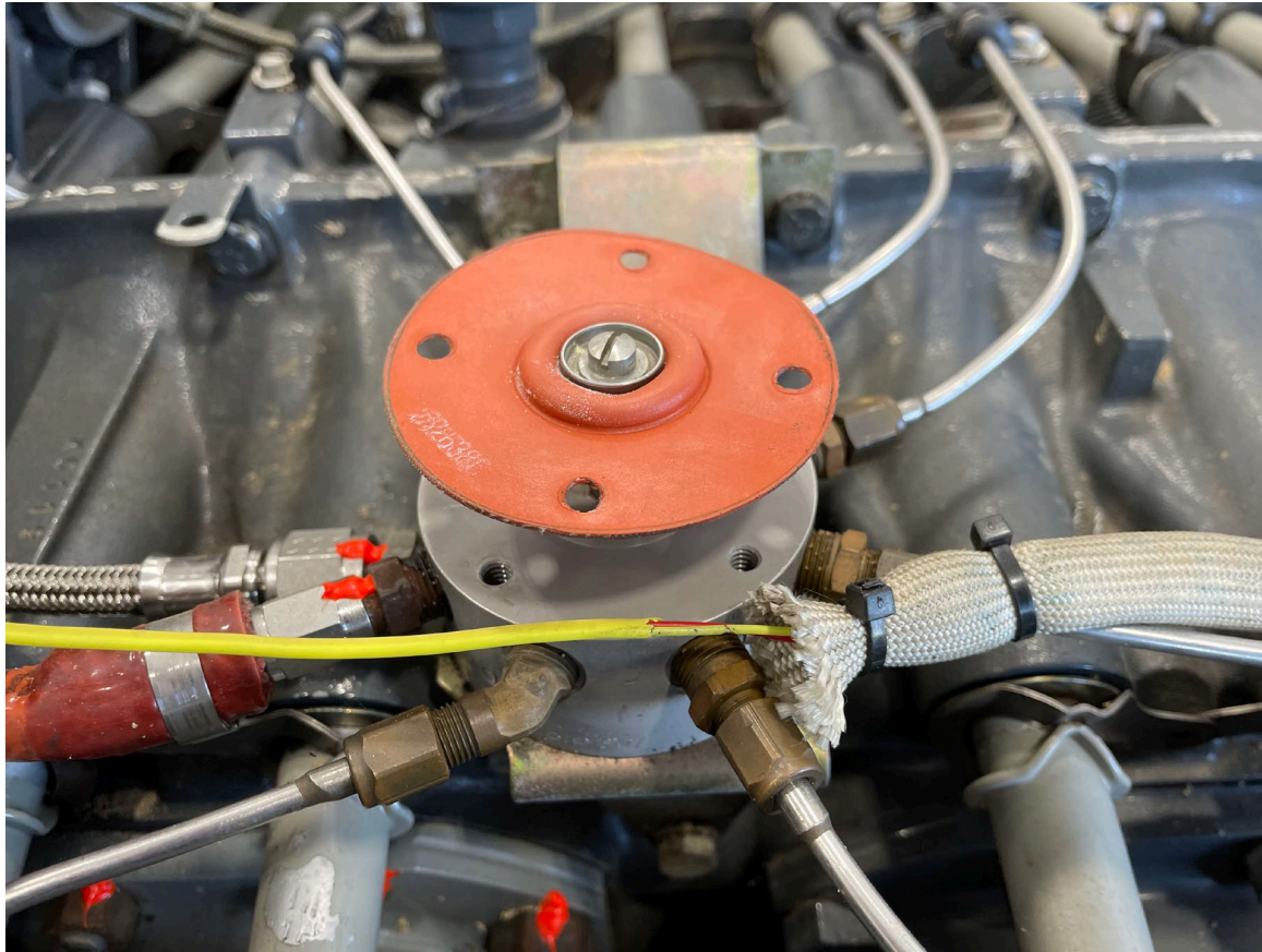
Photograph 5 - Fuel Manifold (NTSB Photo)
