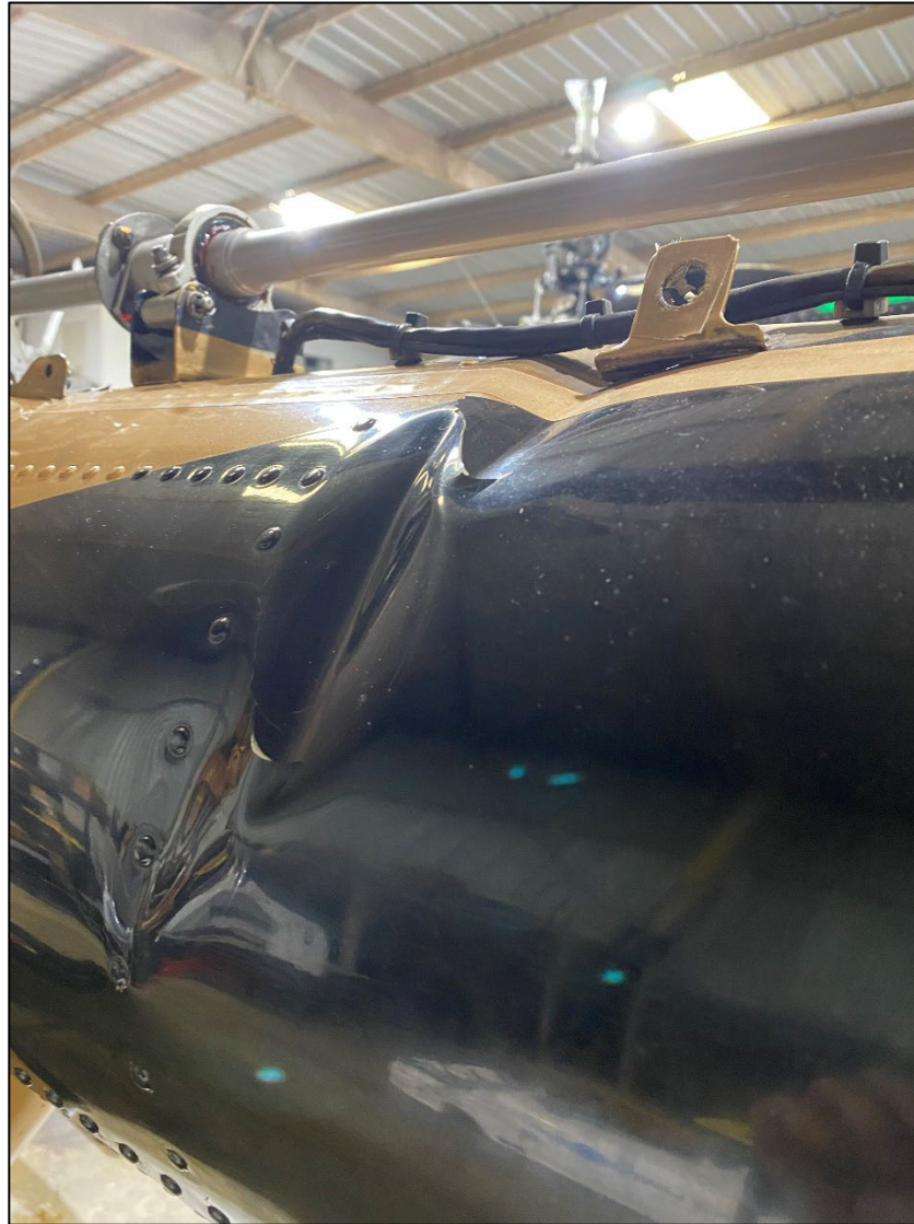
Photograph 2 - Image of the substantially damaged tail boom (Courtesy of FAA)
