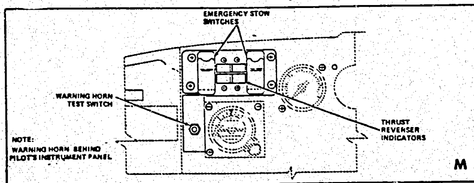
PILOT'S INSTRUMENT PANEL
