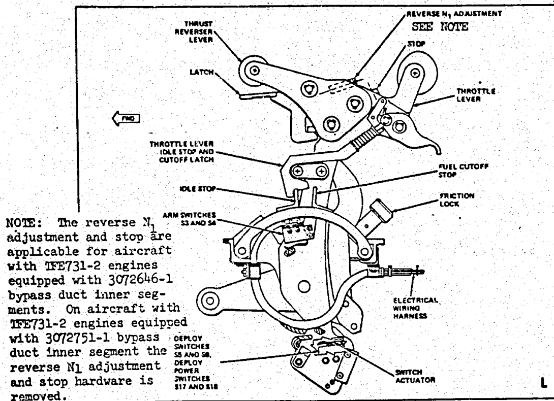
THROTTLE QUADRANT
