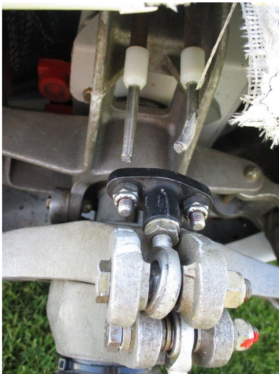
Photo 3 – Fractured Control Linkage at Main Rotor Hub (Cyclic) (FAA)
