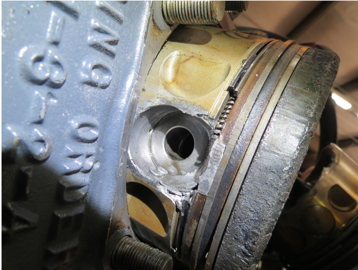
Photograph 3 - No. 2 Cylinder Piston Pin Plug Damage (Lycoming)
