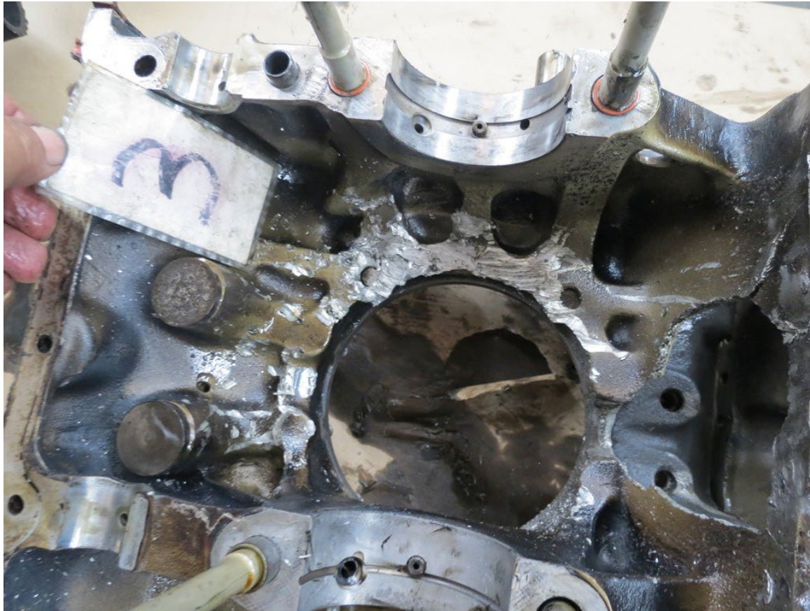
Photograph 4 - Internal Damage to Crankcase (Lycoming)
