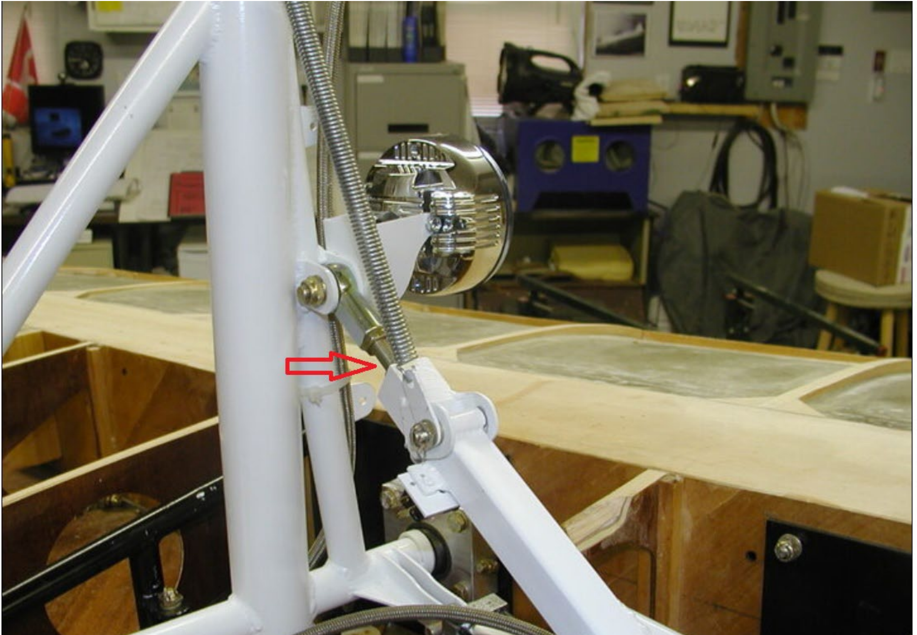
Photo 5 – View of Landing Gear Assembly, After Repairs. Arrow Points to Replaced Lock (Courtesy of Pilot)
