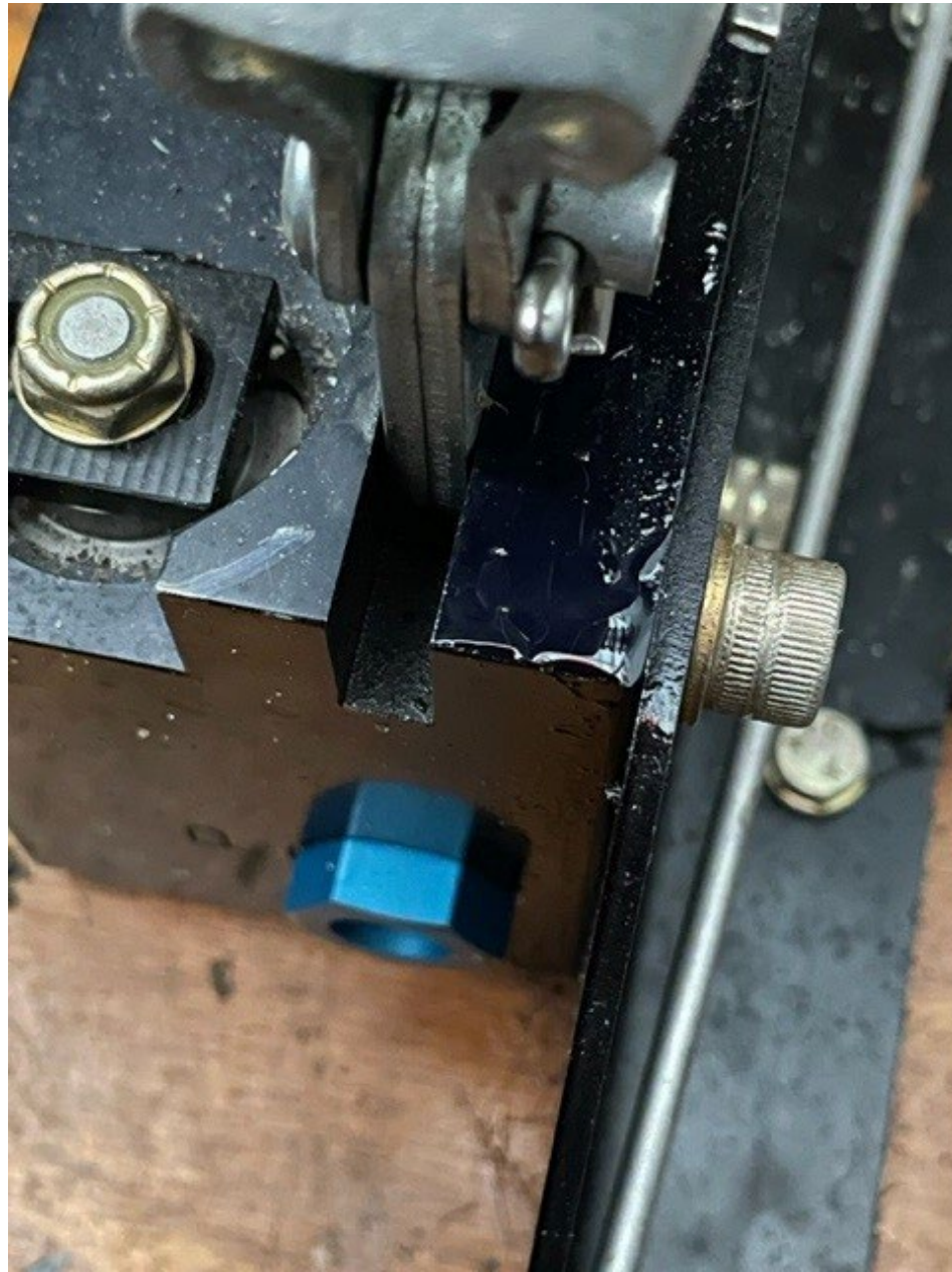
Photo 2 – View of hand pump showing minor leakage (FAA Photo)
