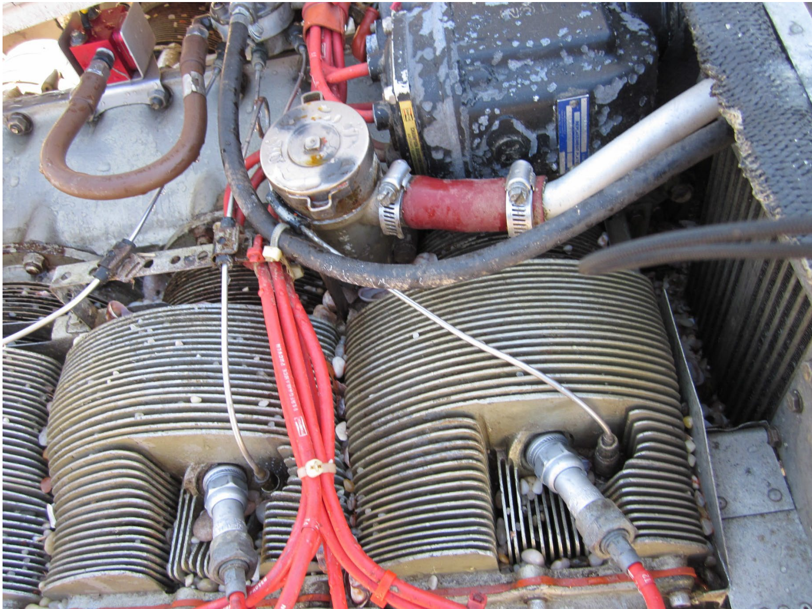
Photo 3 – Engine (FAA)
