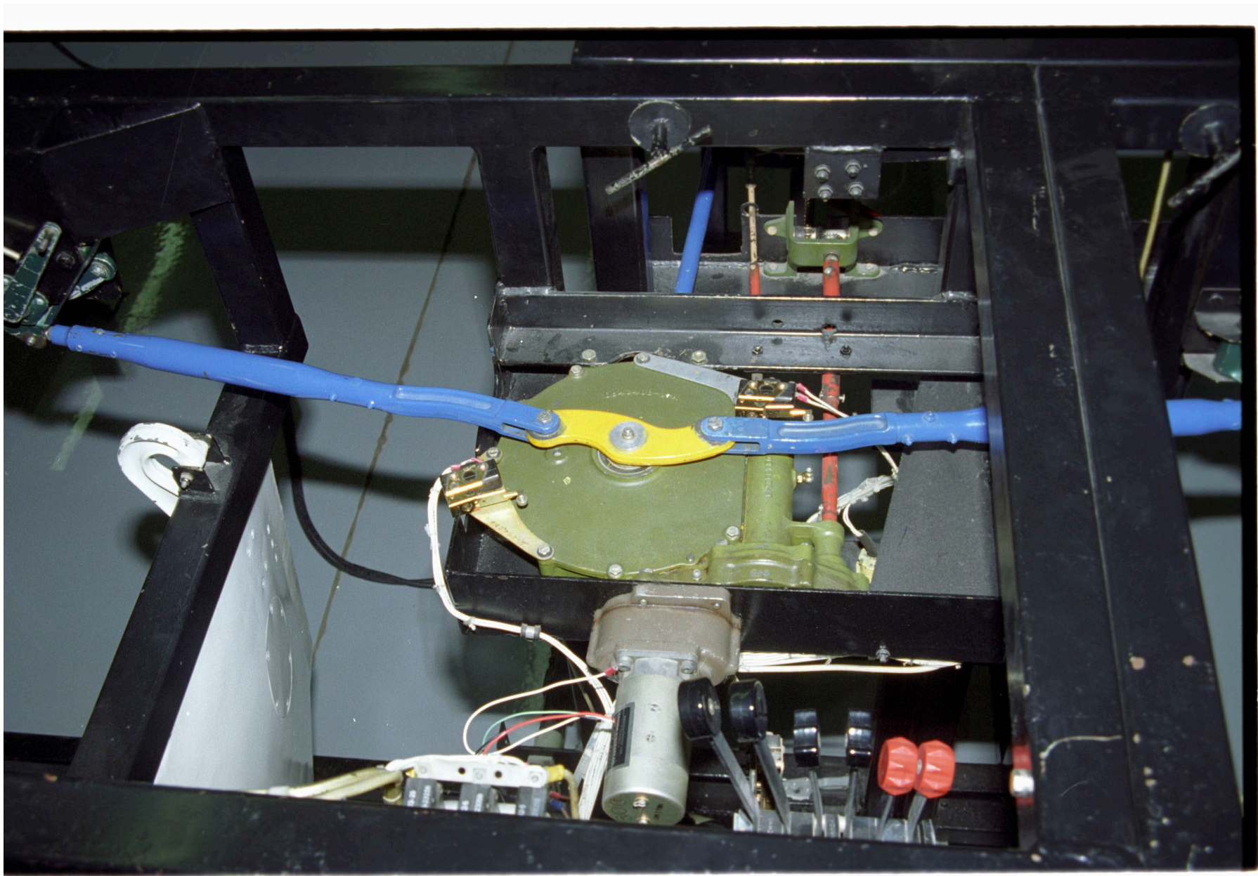
Photo 6 – View of Exemplar Landing Gear Motor in Extended Position (Textron)
