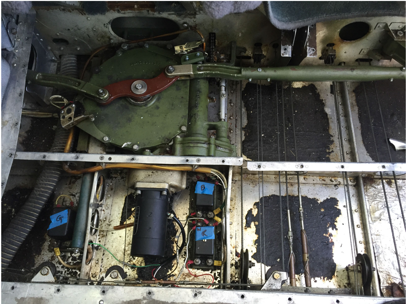
Photo 7 – View of Landing Gear Motor and Damaged Switch from ERA16LA271 (FAA)
