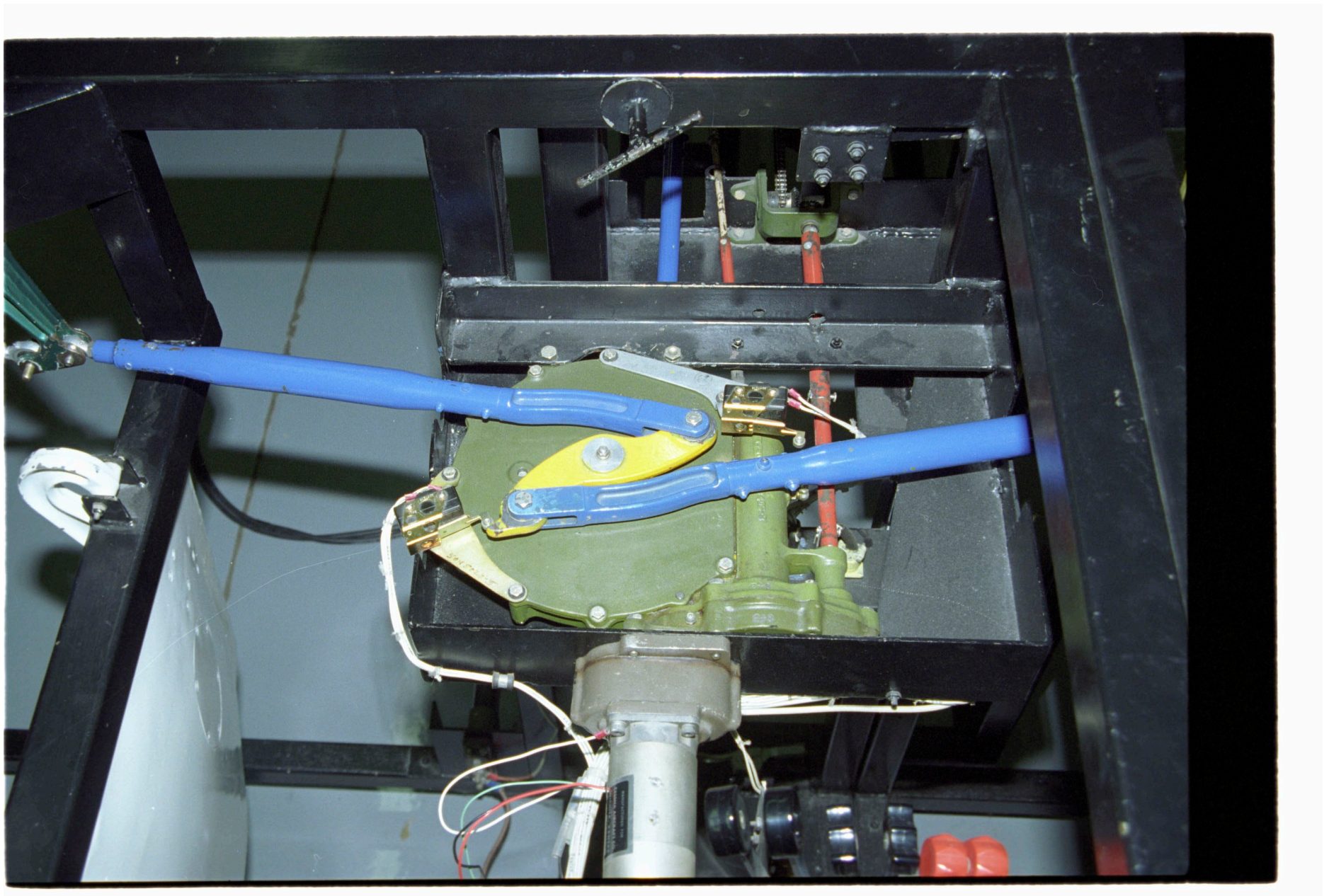
Photo 5 – View of Exemplar Landing Gear Motor in Retracted Position (Textron)
