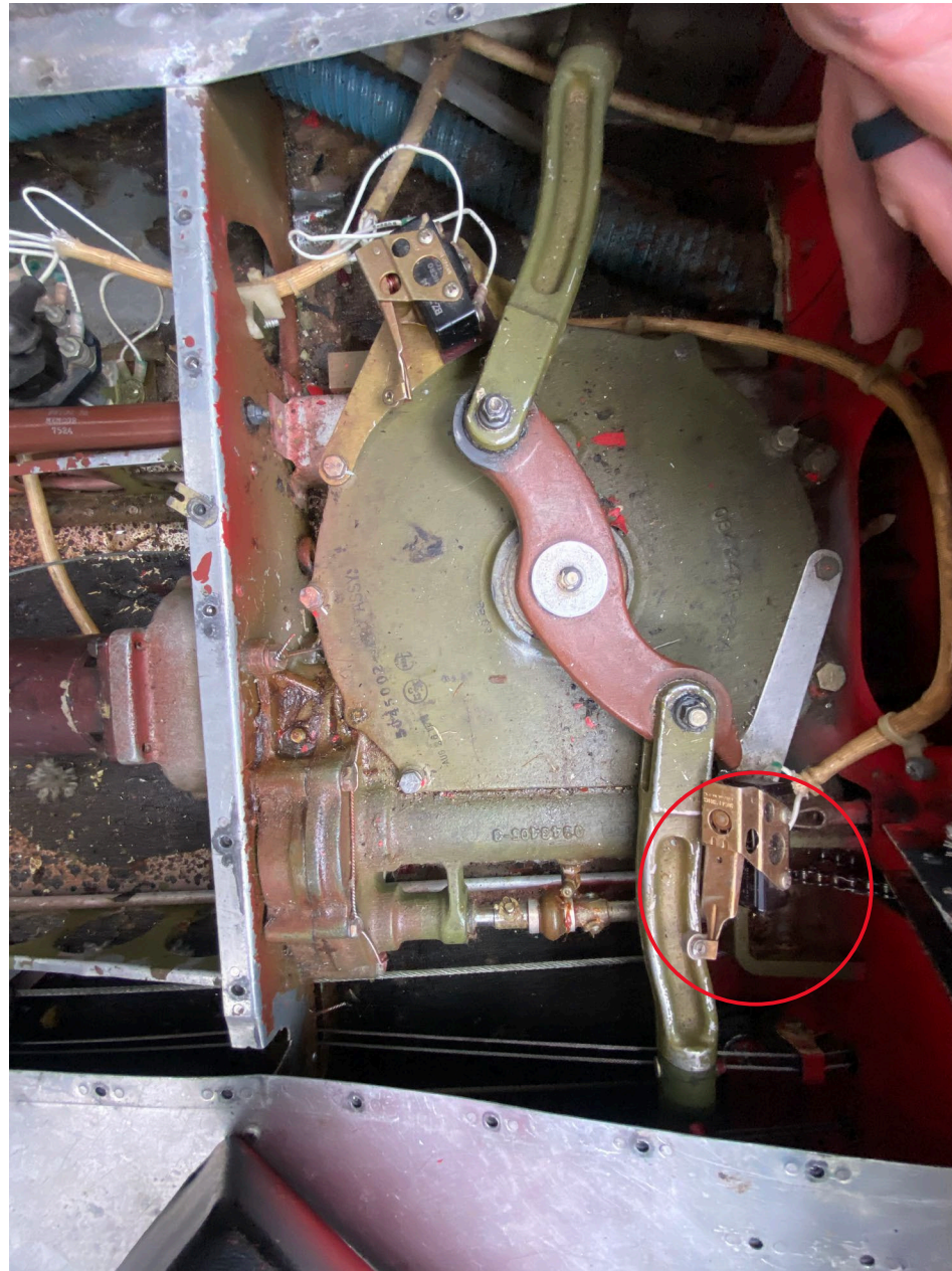
Photo 2 – View of Upper Bellcrank Overtravel and Damaged Down-Limit Switch (Thoroughbred Aviation)
