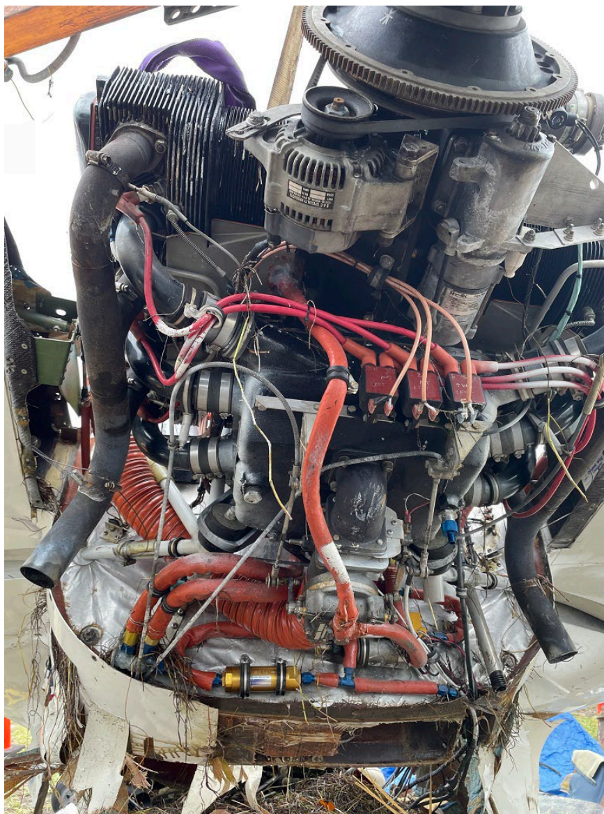
Photograph 4 - Underside of Engine (Courtesy of FAA)
