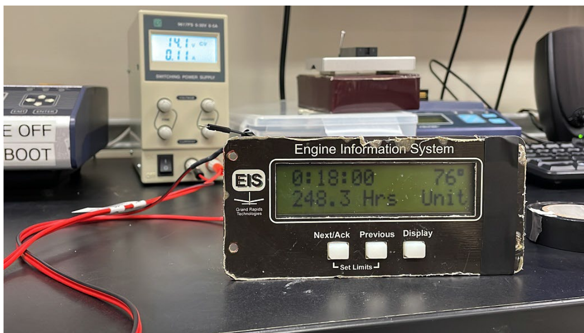
Photograph 5 - EIS Test (Courtesy of NTSB)
