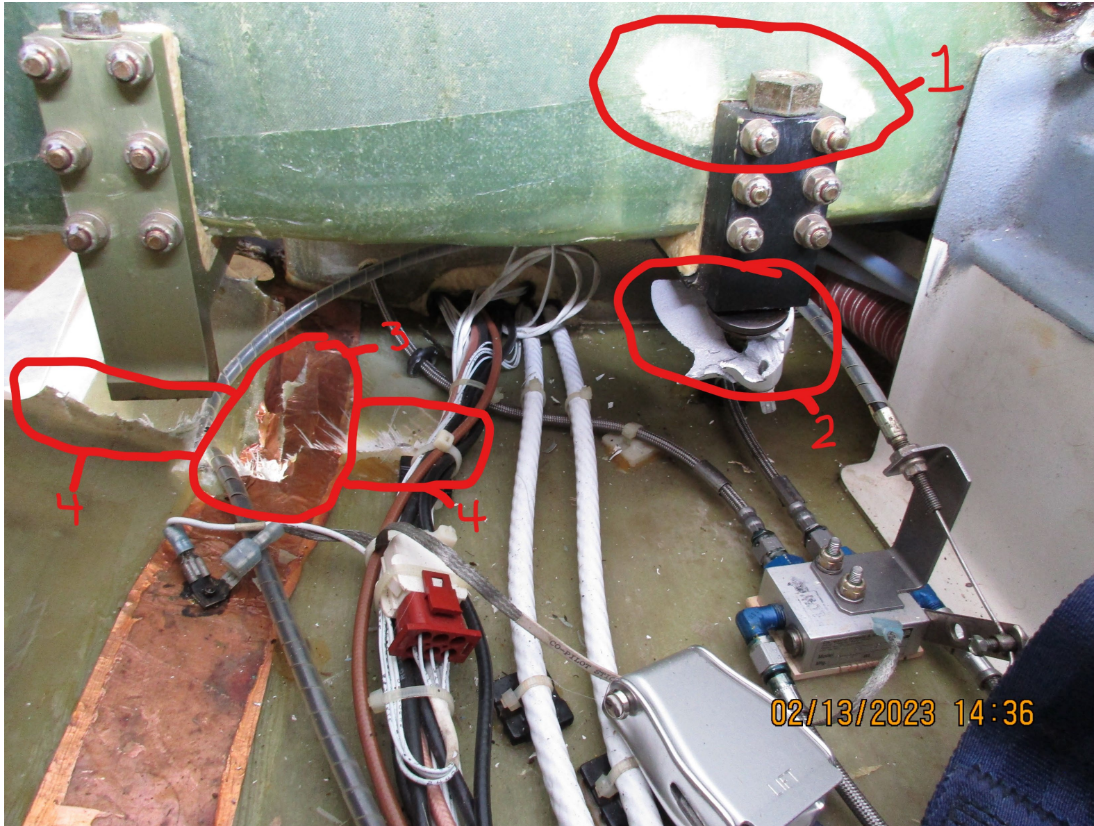
Photo 1: Overview of the airplane center spar delamination damage (red circled #1) (Photo Courtesy of FAA)
