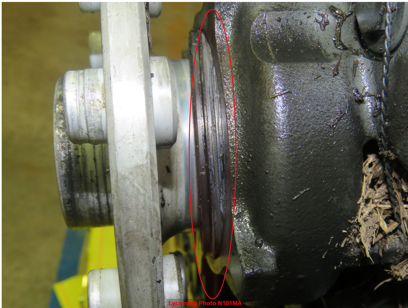
Photo 7 – View of Extruded Crankshaft Nose Seal (Lycoming)
