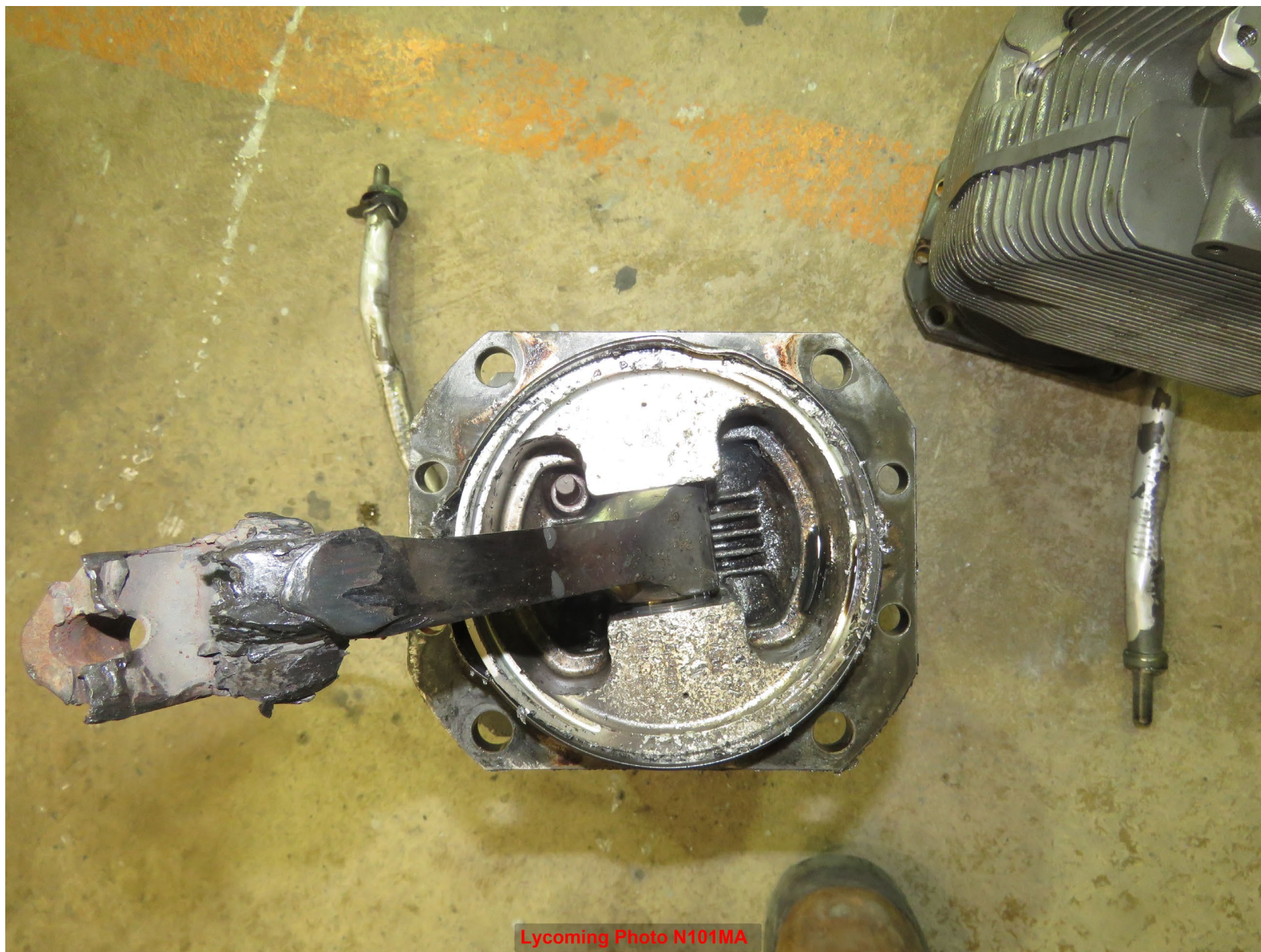
Photo 5 – View of #5 Piston with Broken Connecting Rod inside #5 Cylinder (Lycoming)
