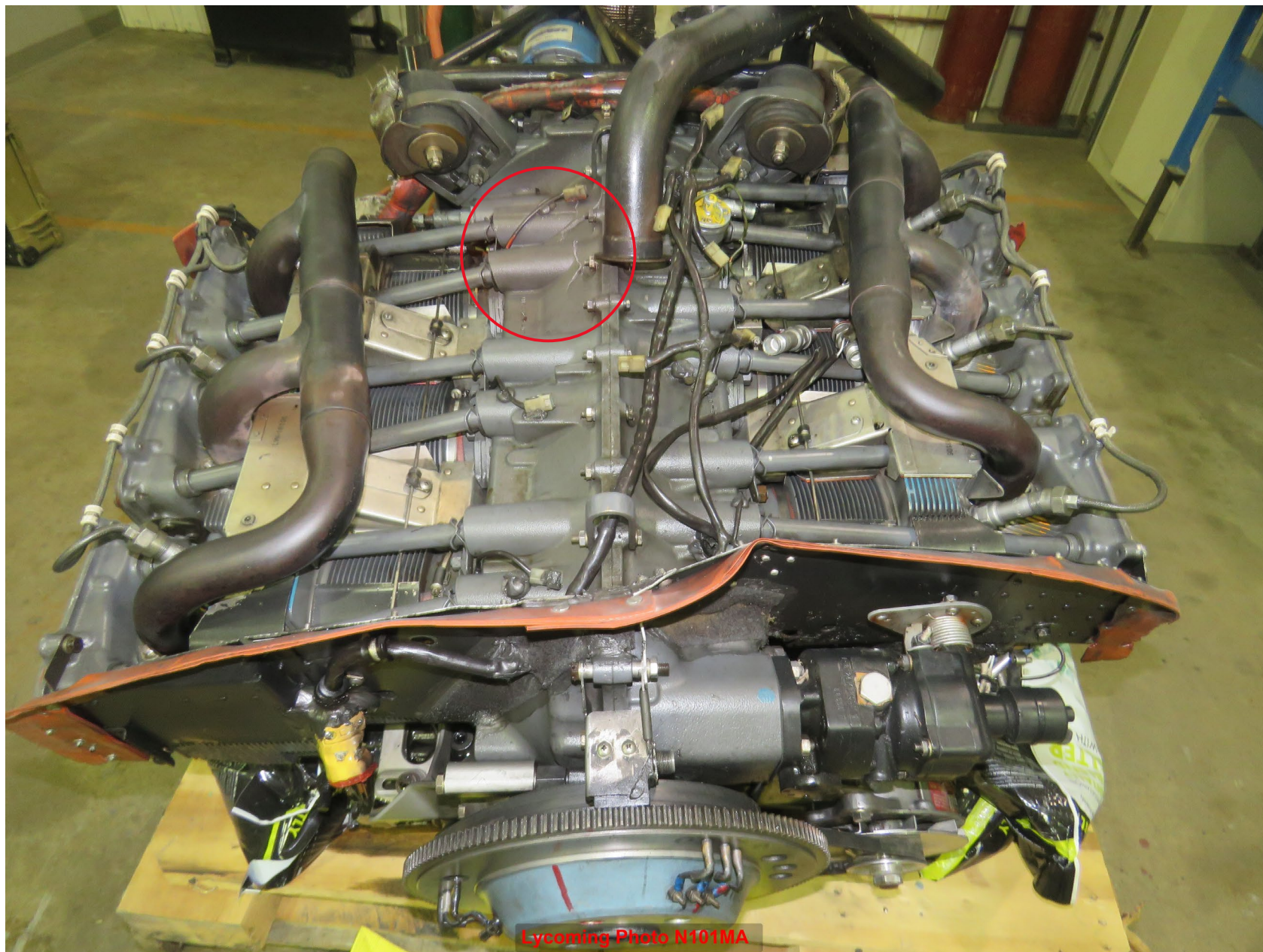
Photo 4 – View of Engine Uncrated in Examination Room (Lycoming)
