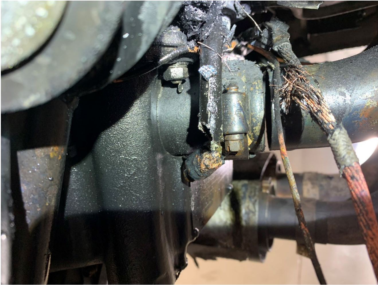
Photograph 3 - View of alternator wire damage. (Courtesy of FAA)
