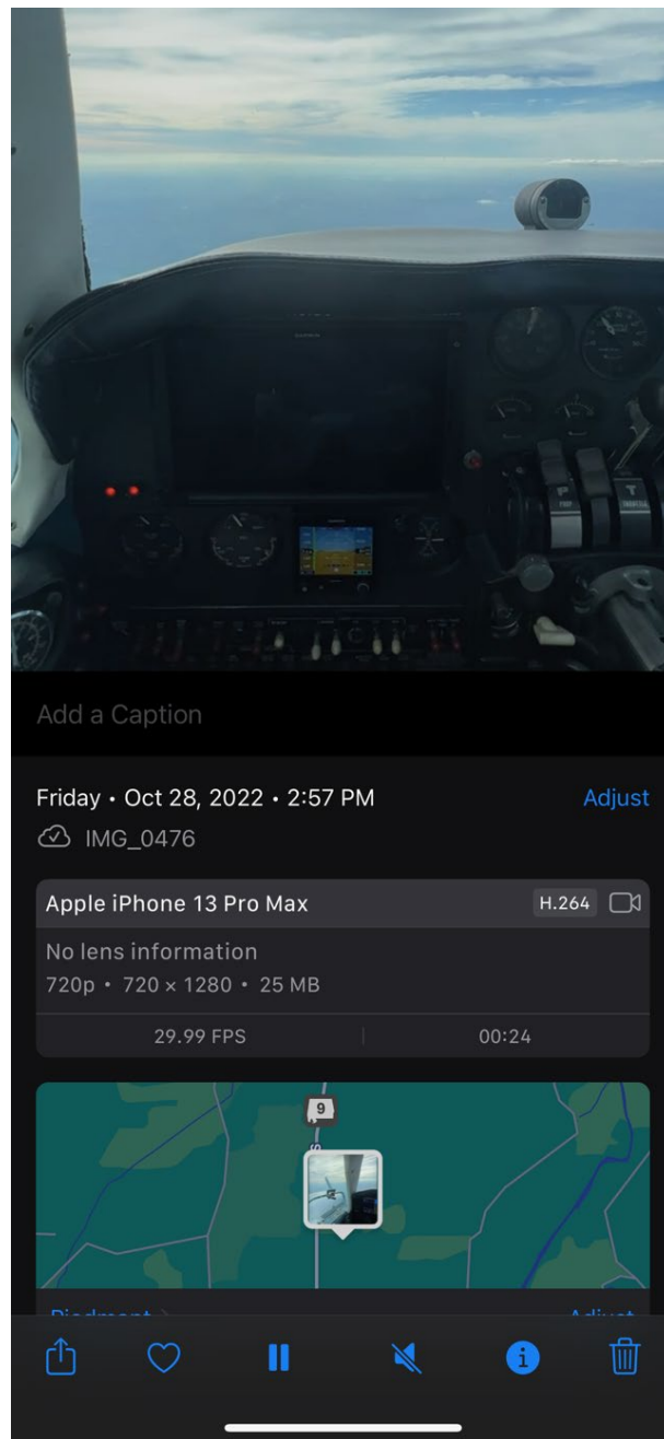
Photo 1: iPhone Photo taken on October 28, 2022 showing both alternator lights illuminated (left, center of photo).
