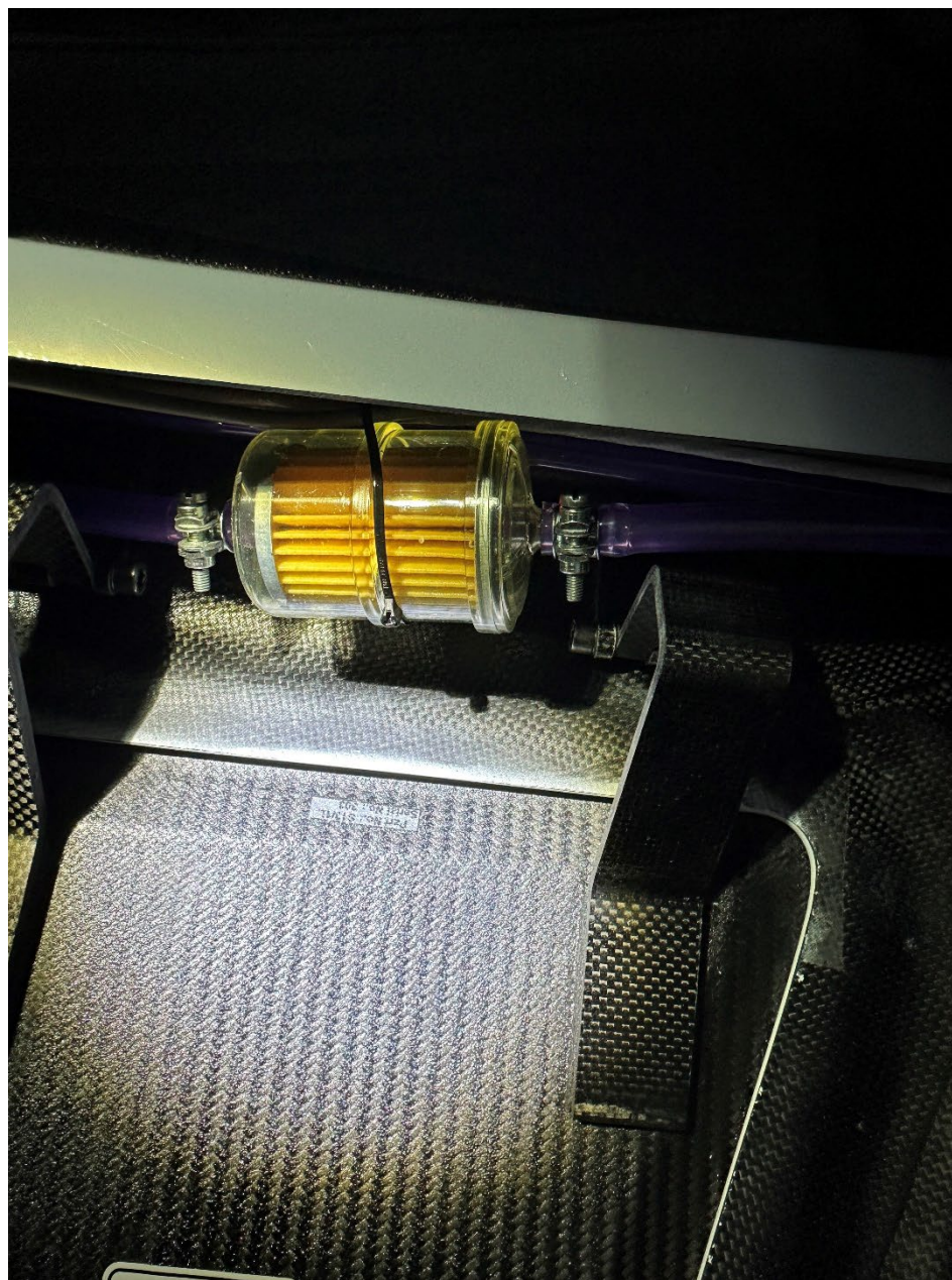
Photo 8 – In Line Fuel Filter Showing No Fuel (Right Rudder Aviation Photo)
