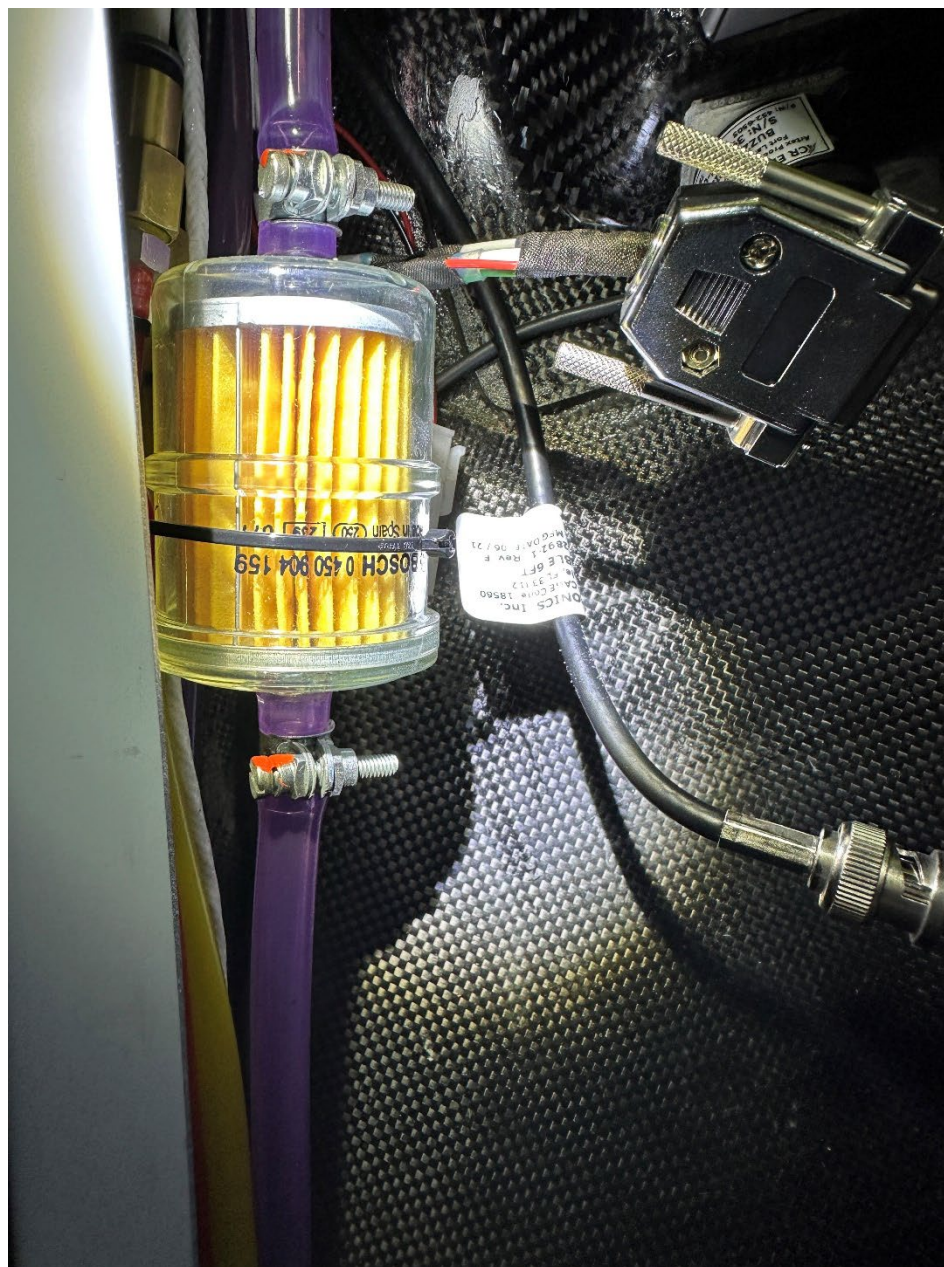
Photo 7 – In Line Fuel Filter Showing No Fuel (Right Rudder Aviation Photo)
