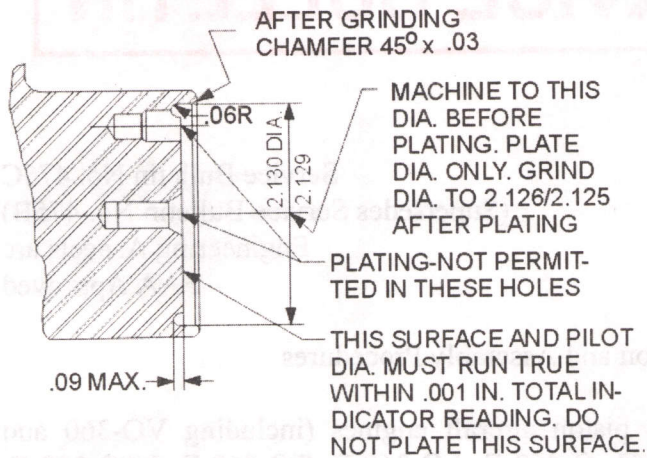
Figure 1. Details for Repairing Pilot Diameter of Crankshaft
