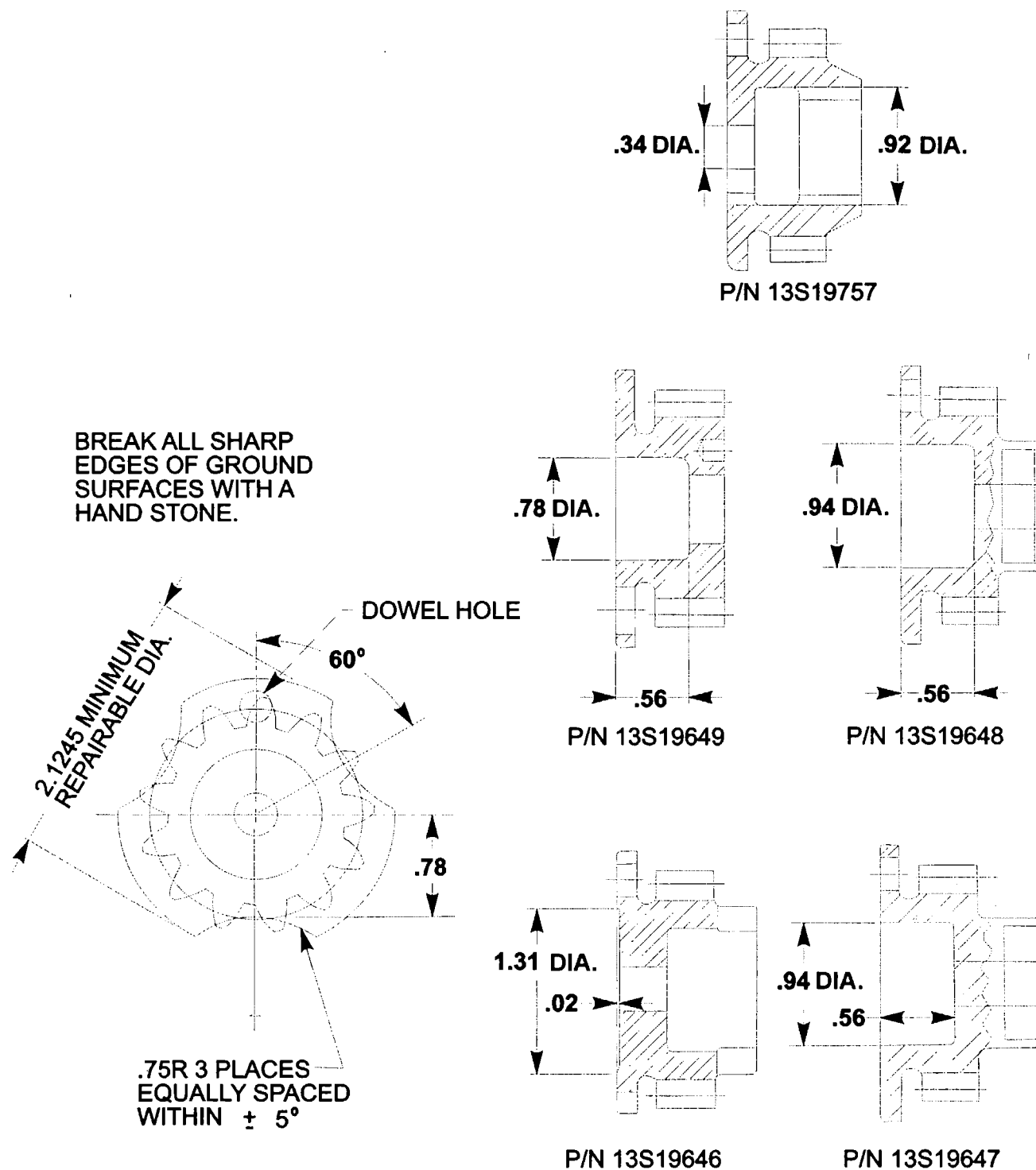
Figure 5. Details for Rework of Crankshaft Gears to Current Configuration
