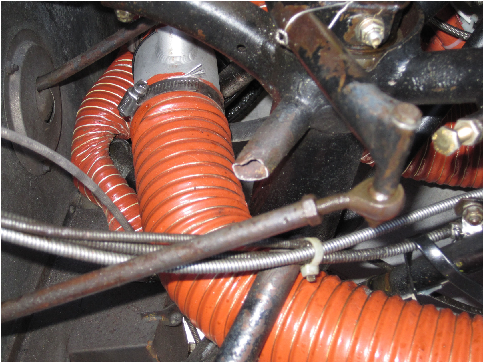
Photo 2 – Broken Engine Mount (FAA Photo)
