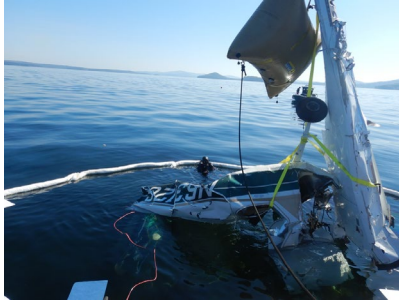
Photo 1: Airplane Wreckage Being pulled from the Lake (Textron)
