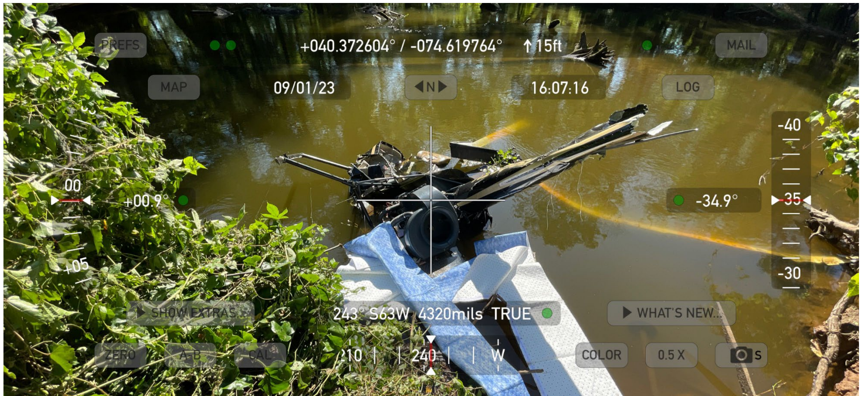
Photograph 1 - View of wreckage resting in water with location details. Note oil mats to prevent fuel and oil from escaping into waterway. (NTSB IIC)
