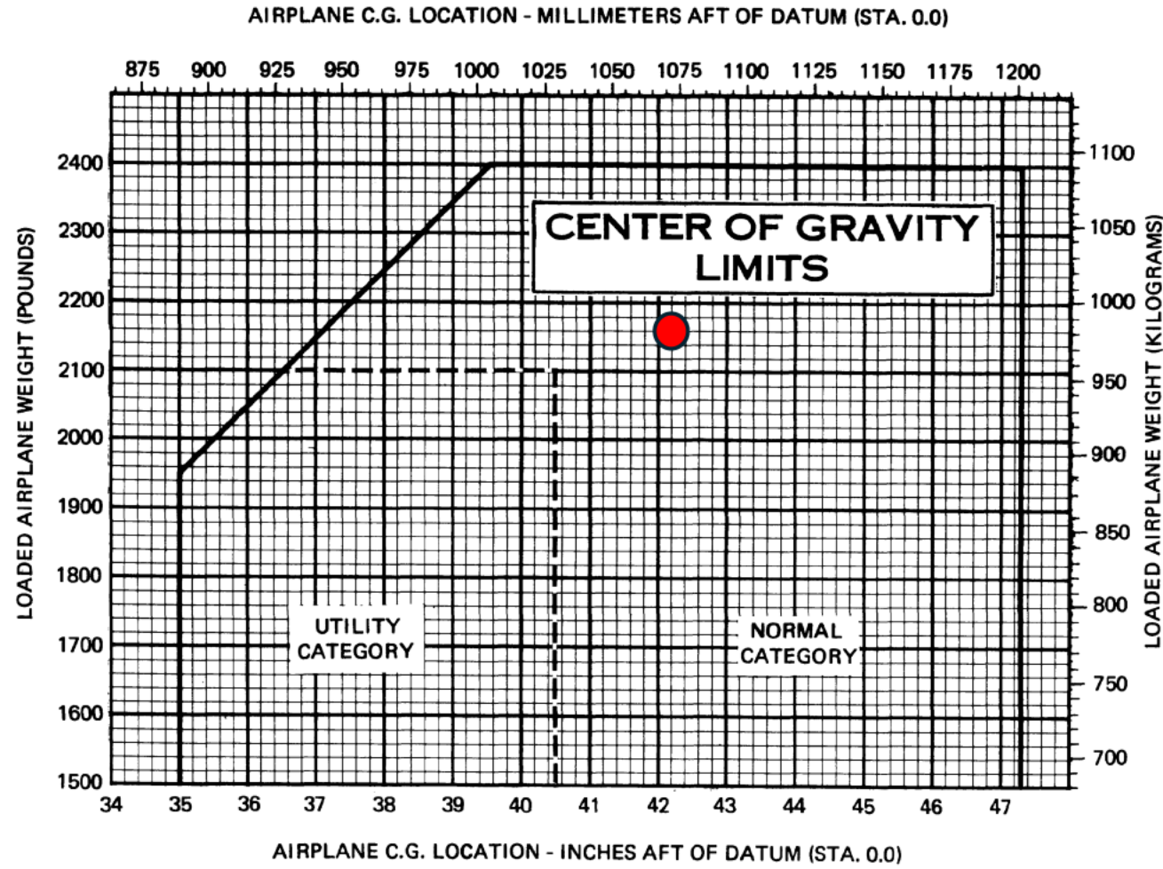
Figure 6-8. Center of Gravity Limits
