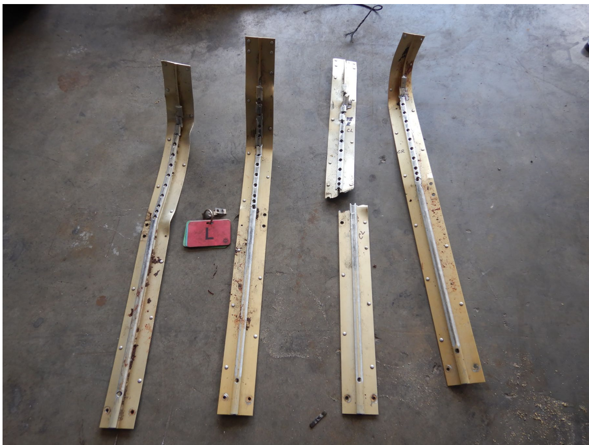
Photograph 7 - View of seat tracks during examination. (Courtesy of Textron)
