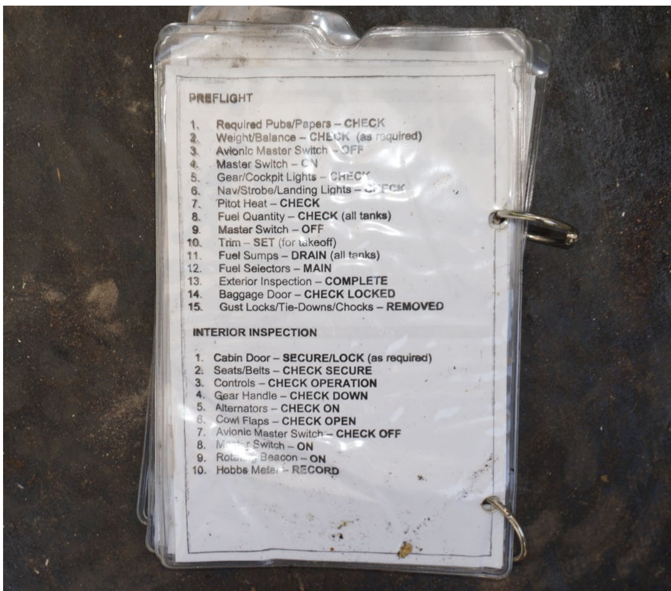
Photograph 22 - Preflight Checklist
