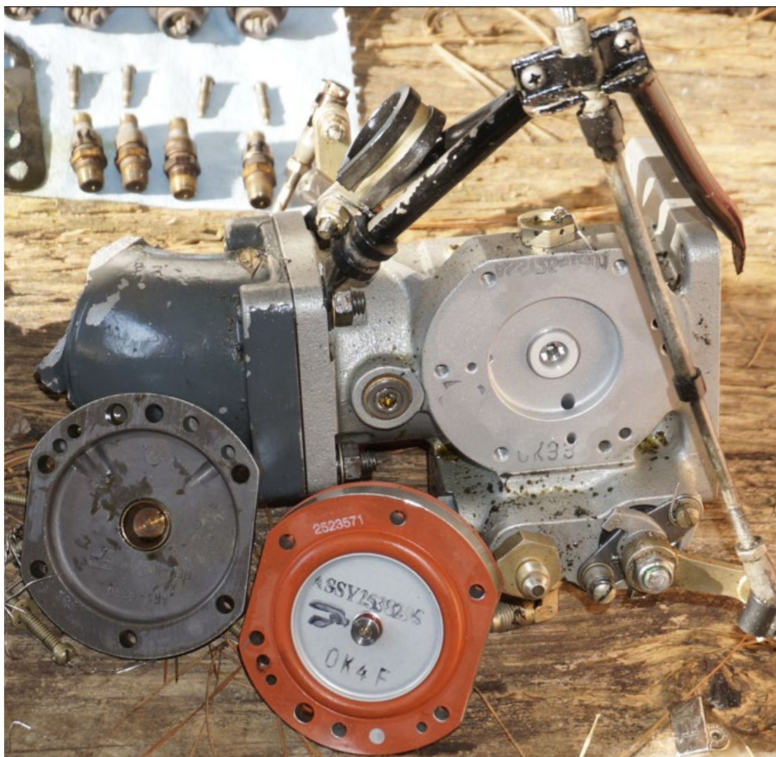
Photograph 17 - Right Engine Fuel Servo
