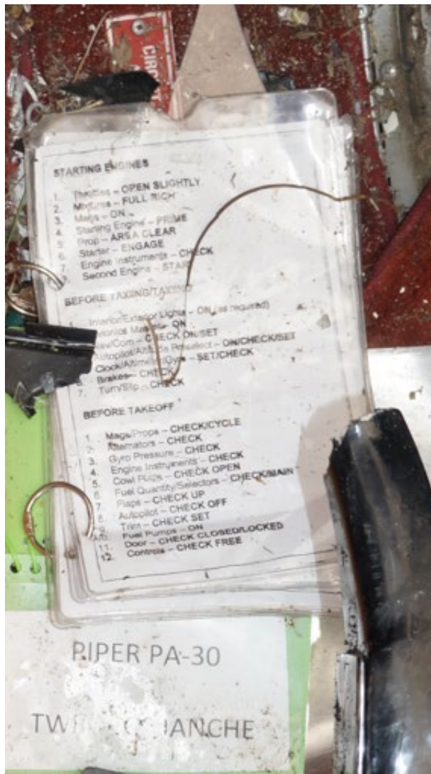
Photograph 15 - Before Takeoff Checklist (As Found)
