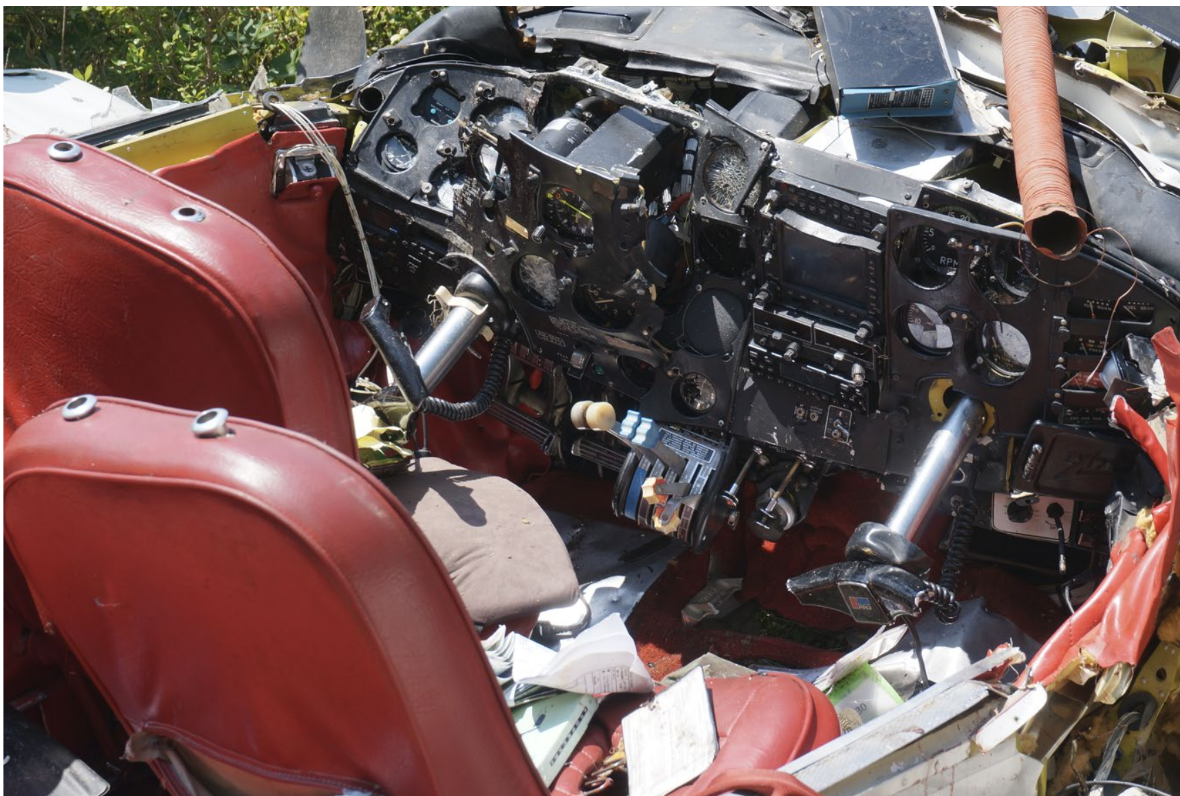
Photograph 7 - Instrument Panel
