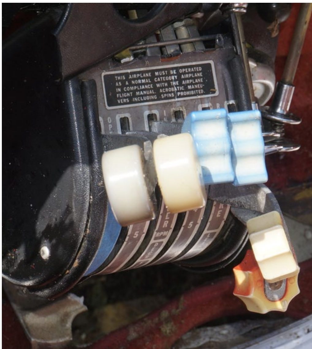
Photograph 11 - Throttle Quadrant
