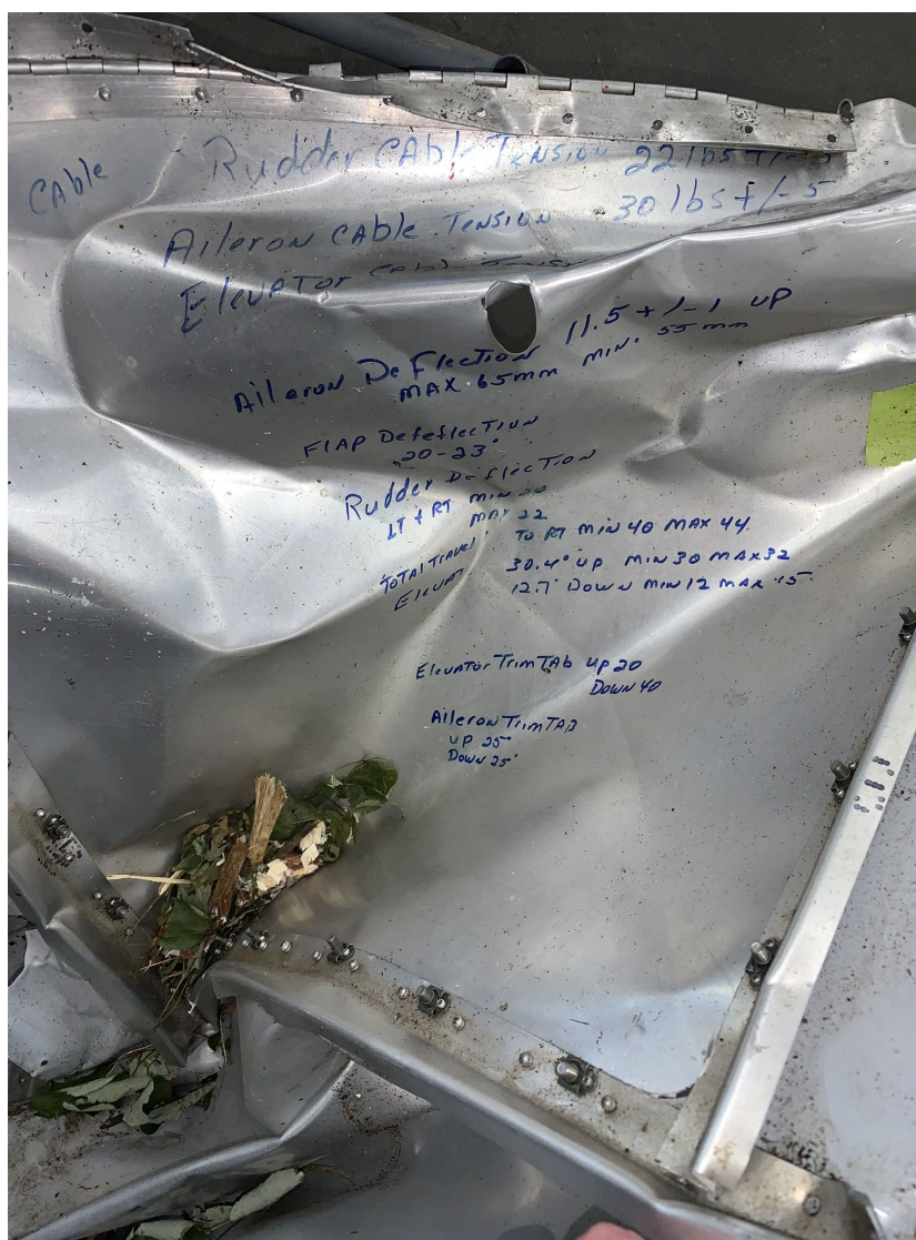
Photograph 4 -Handwritten notes on fuselage about flight control settings. (NTSB)
