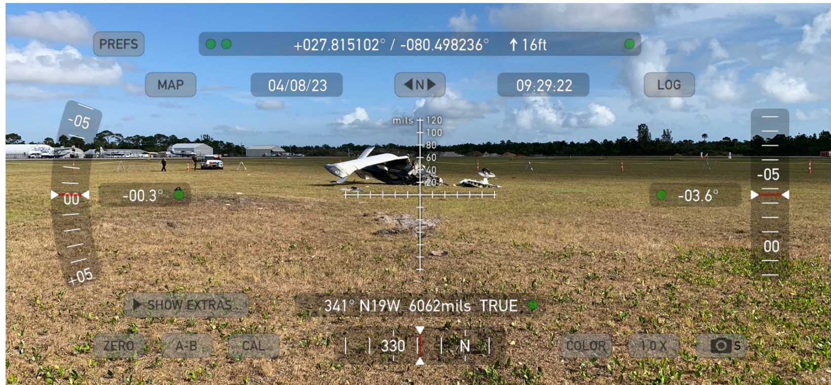
Photograph 7 - Overall view of accident site taken from initial ground impact point showing heading, lat/log and elevation.
