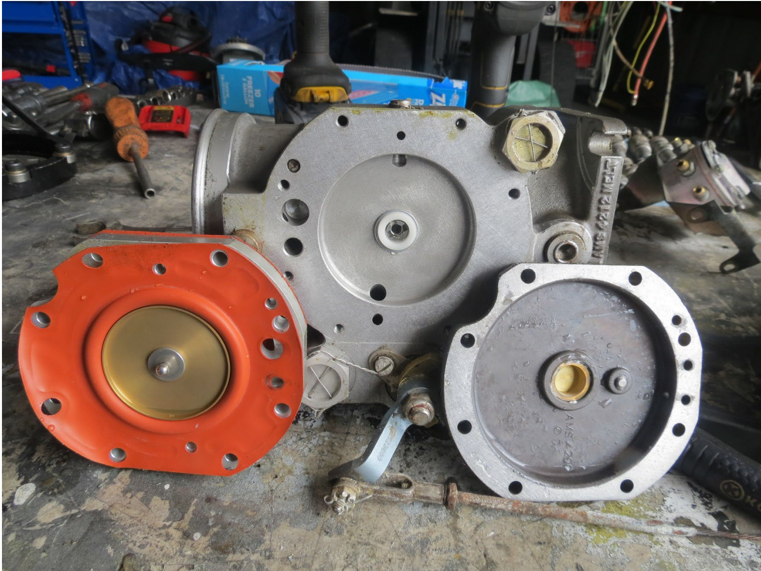
Photograph 21 - Interior of Fuel Servo (Courtesy of Lycoming Engines)
