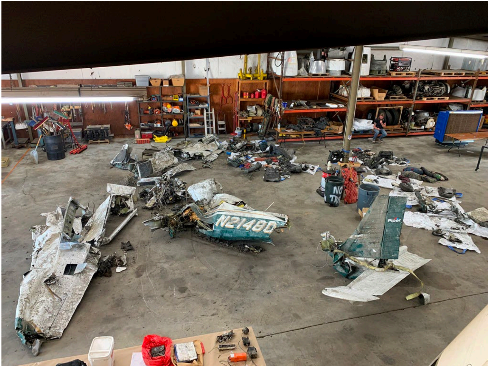
Photo 5 – Overhead View of Wreckage
