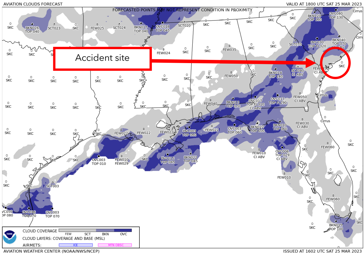
Figure 6. GFA Aviation Clouds Forecast valid at 1400 EDT with forecast issued at 1202 EDT.
