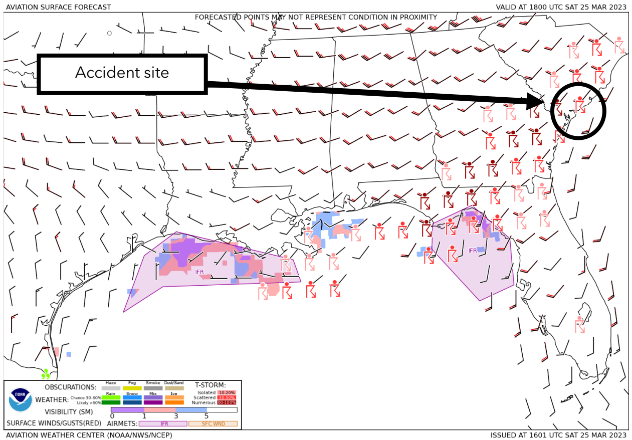
Figure 3. GFA Surface Forecast valid at 1400 EDT with forecast issued at 1201 EDT.
