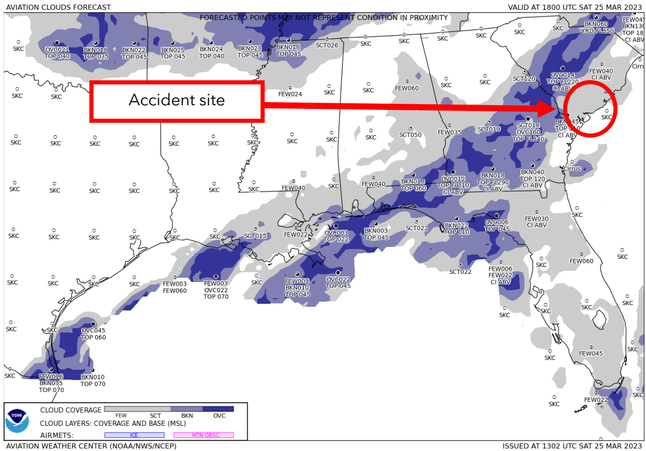
Figure 5. GFA Aviation Clouds Forecast valid at 1400 EDT with forecast issued at 0902 EDT.
