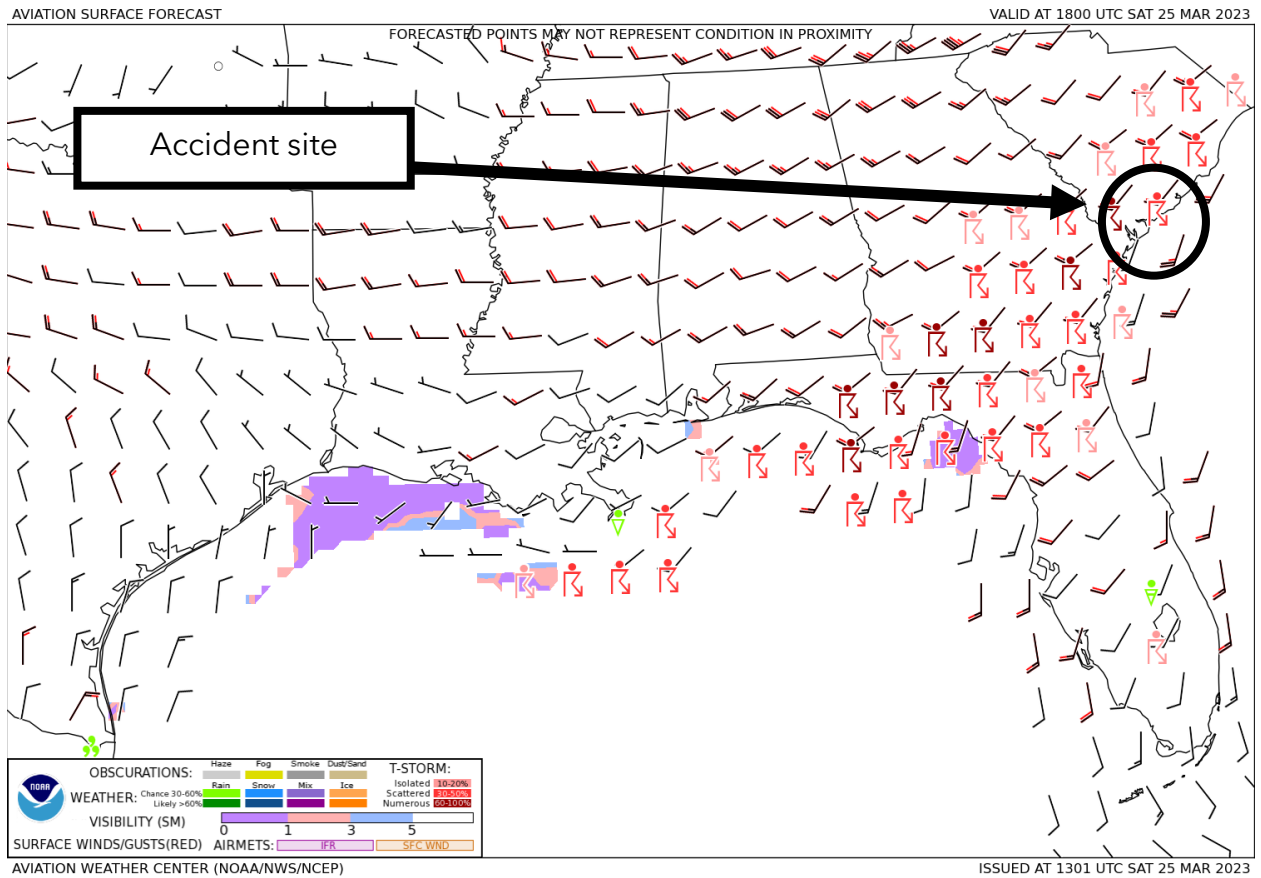
Figure 2. GFA Surface Forecast valid at 1400 EDT with forecast issued at 0901 EDT.
