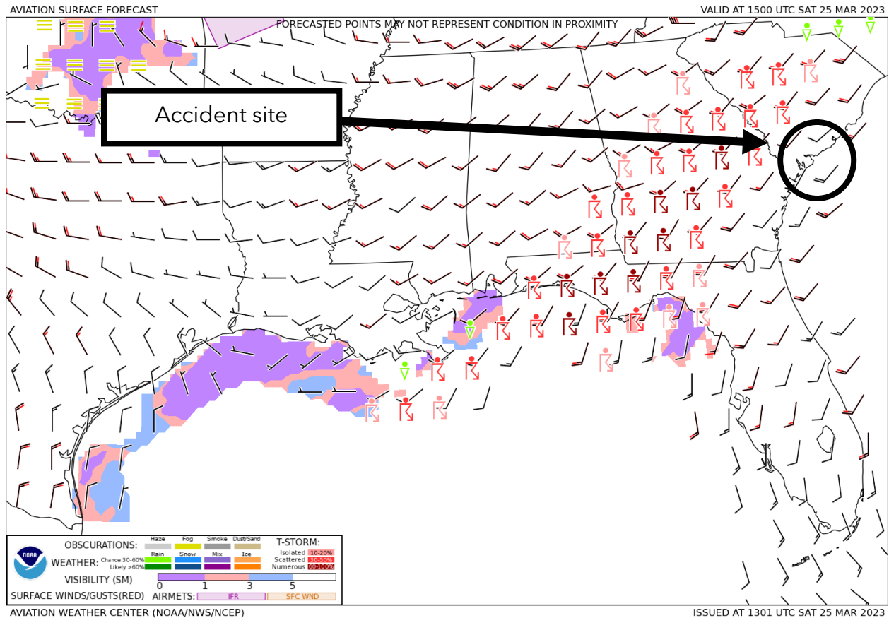
Figure 1. GFA Surface Forecast valid at 1100 EDT with forecast issued at 0901 EDT.
