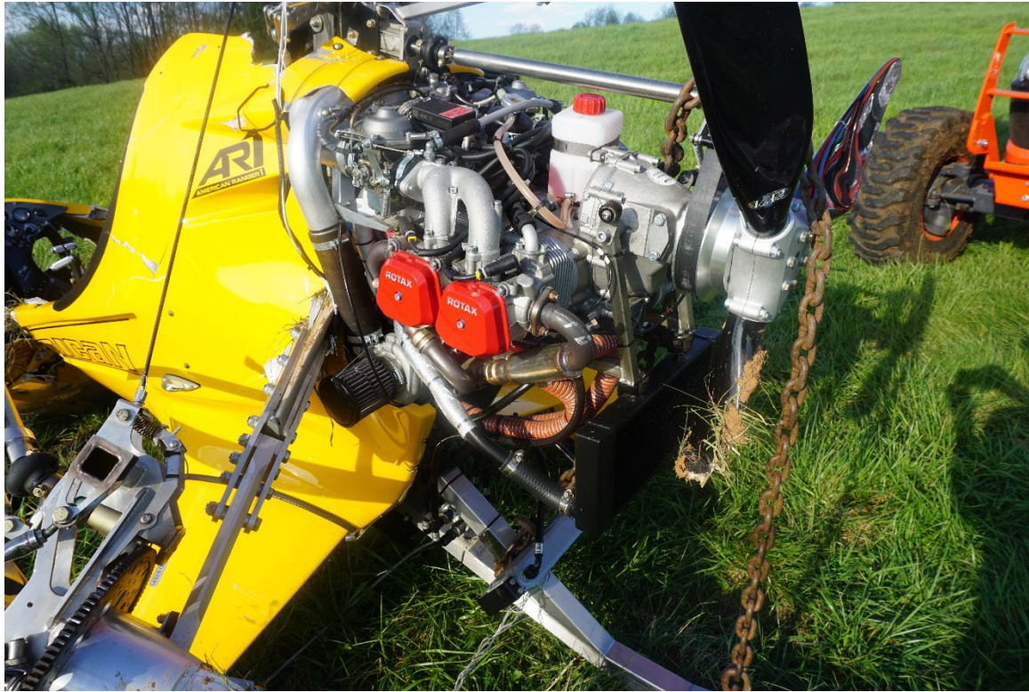
Photograph 4 - Yellow Gyrocopter main wreckage engine view
