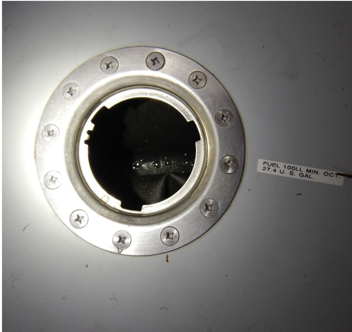
Photograph 13 - Right wing fuel bladder with no visible fuel
