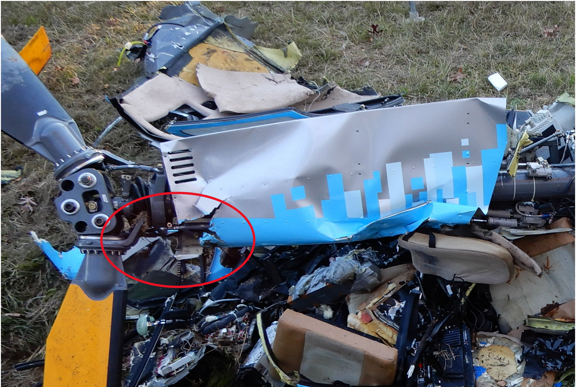
Photo 7 – Main Rotor Hub and Mast (NTSB Photo)
