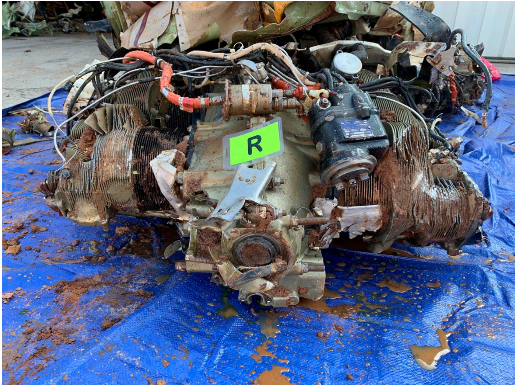
Photo 7 – Right Engine
